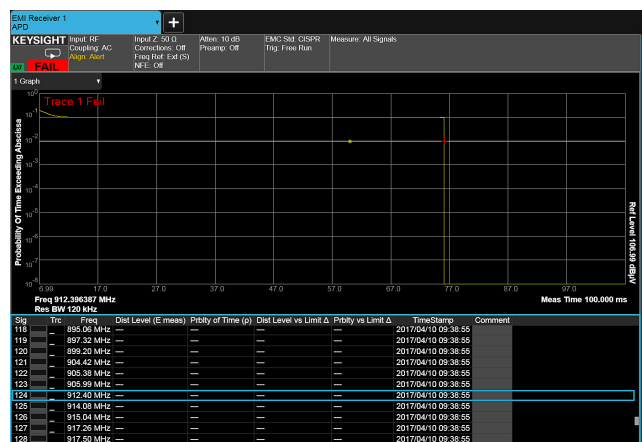
Figure 10. APD measurement example
