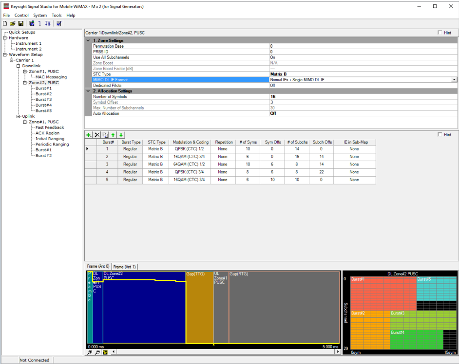
Figure 3. Navigate through the frame elements using the software's tree view in the left panel to quickly customize OFDMA waveforms with multiple zones and data bursts.
