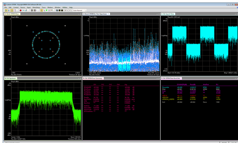
Figure 3. Pre-5G single carrier measurement with 89601B-BHF
