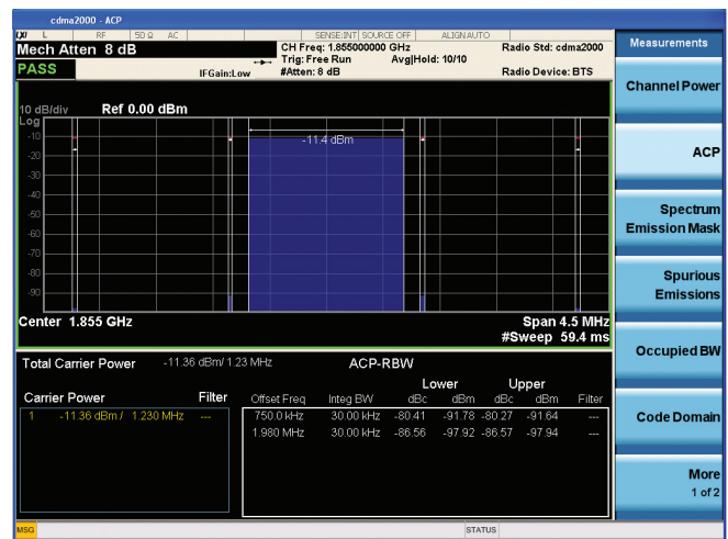
Figure 6. cdma2000 ACP measurement.
