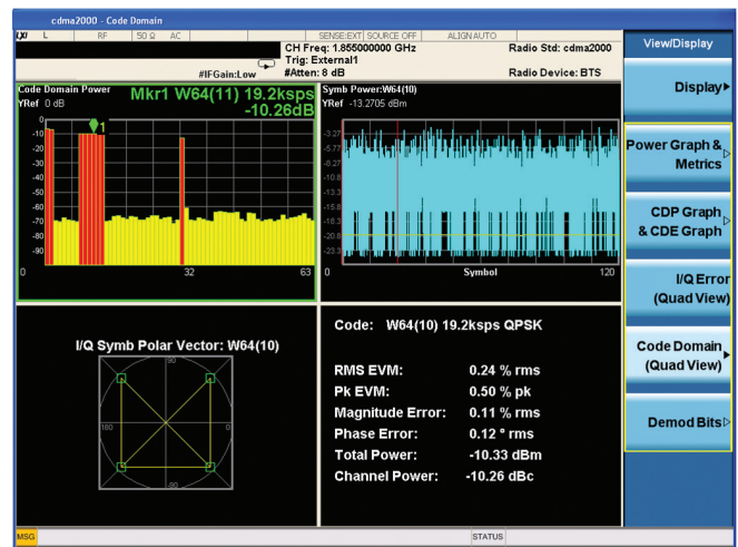
Figure 4. Code Domain Power quad view.
