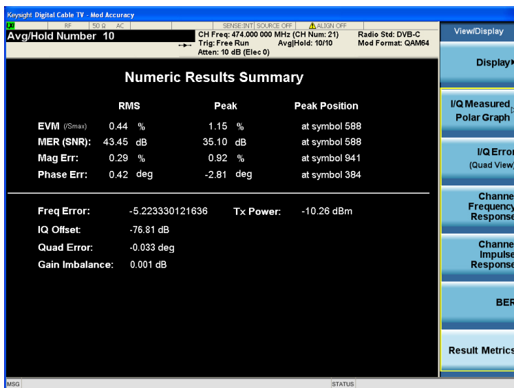
Figure 4. DVB-C result metrics view
