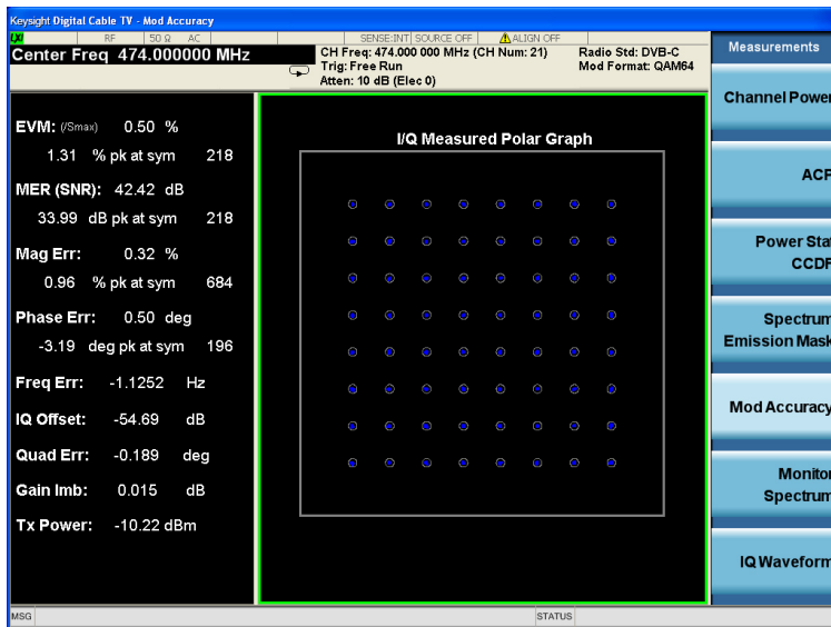
Figure 2. DVB-C constellation and MER results
