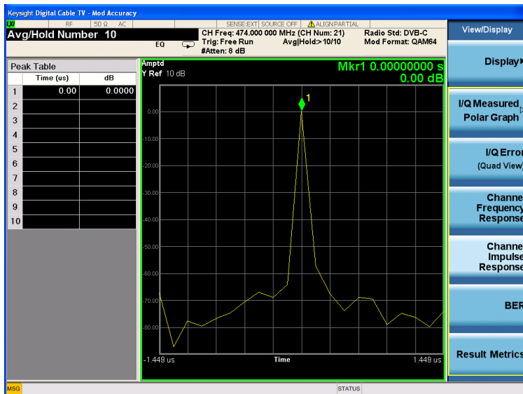
Figure 6. DVB-C channel impulse response view
