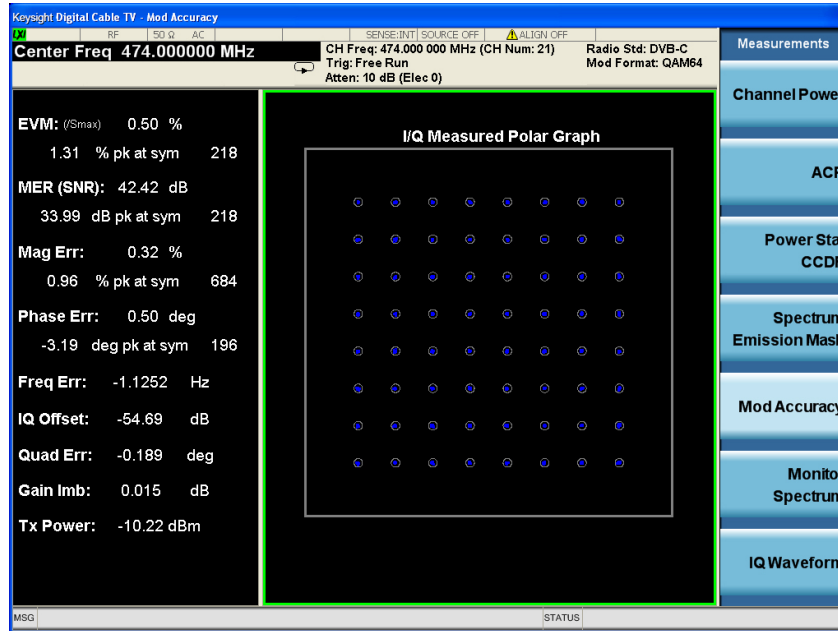
Figure 1. DVB-C modulation accuracy.
