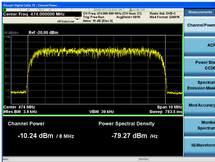
Figure 5. DVB-C channel power
