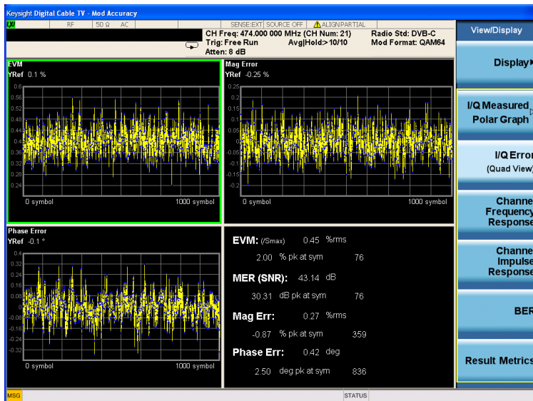
Figure 3. DVB-C IQ quad view
