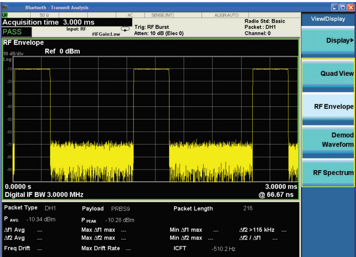
Figure 4. RF envelope view of transmit analysis measurement for the Bluetooth basic rate
