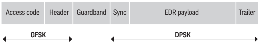
Figure 11. Bluetooth EDR packet format
