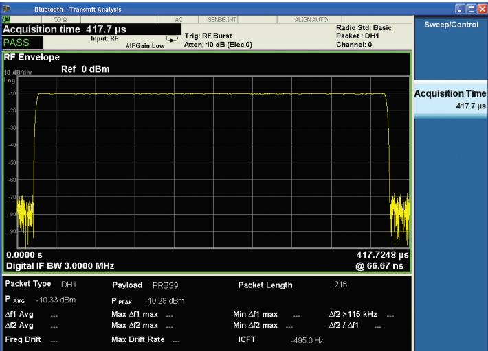
Figure 5. The Bluetooth one burst signal (DH1 packet, PRBS9 as payload and packet length 216 bits)
