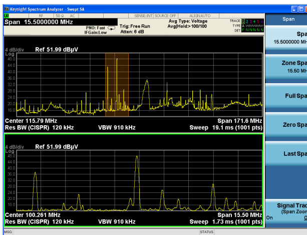
Figure 13. Zone span
