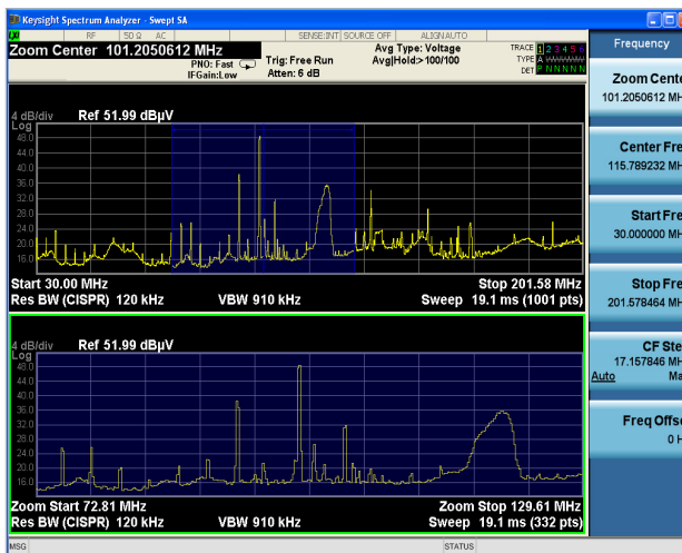
Figure 12. Trace zoom
