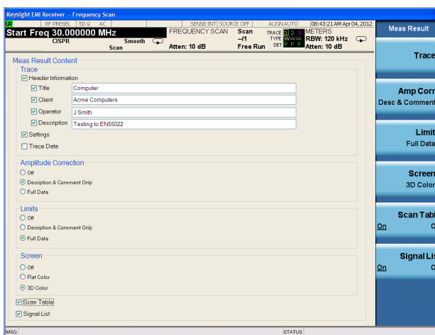
Figure 6. Report generation
