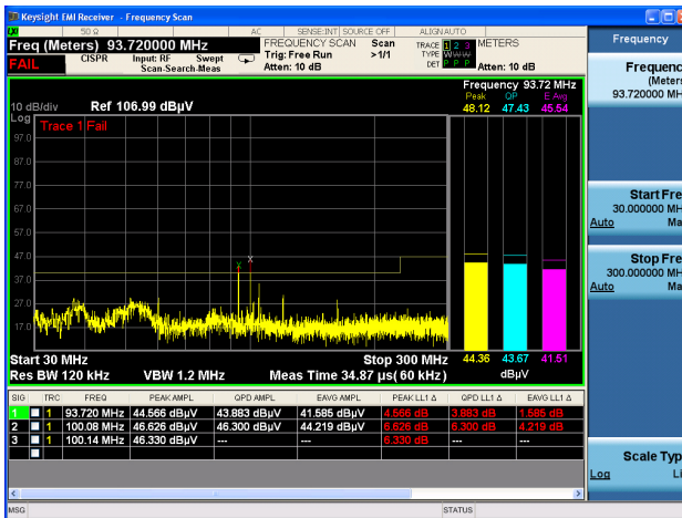
Figure 1. Frequency scan
