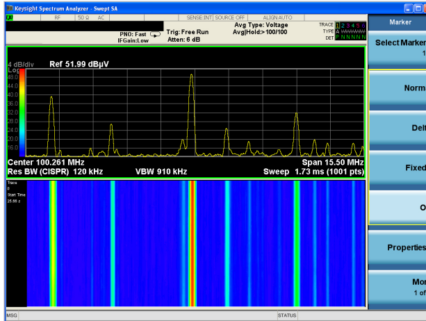
Figure 11. Spectrogram
