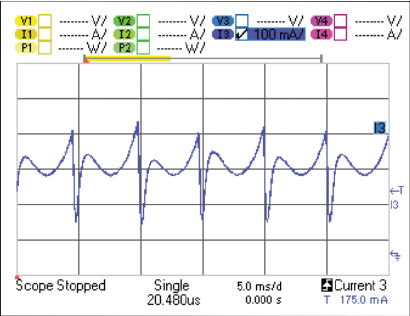
Figure 1. N6705A screen shot of Scope View
