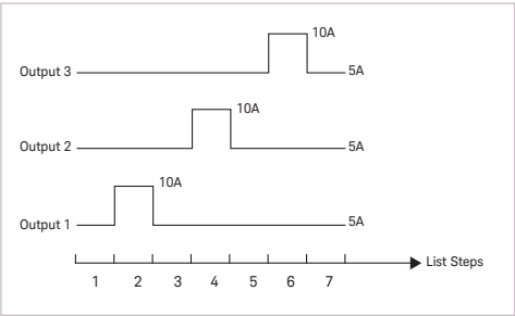
Figure 2. Changing power supply currents sequentially to observe cross regulation.
