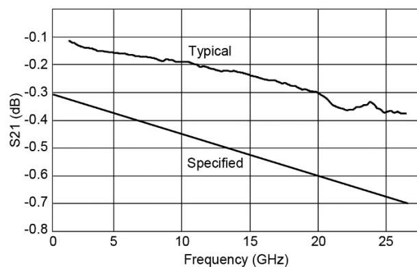
Figure 7. Insertion loss
