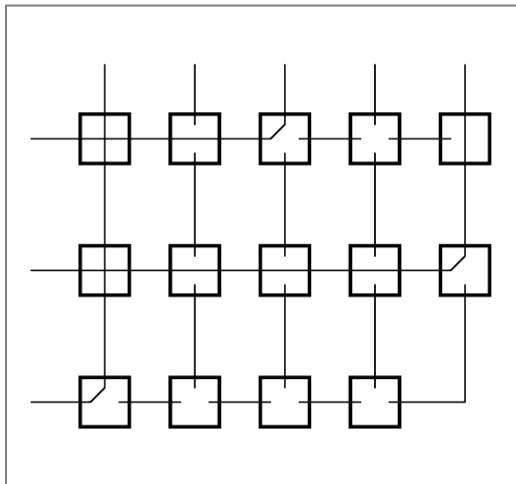
Figure 4. Cross-point matrix
