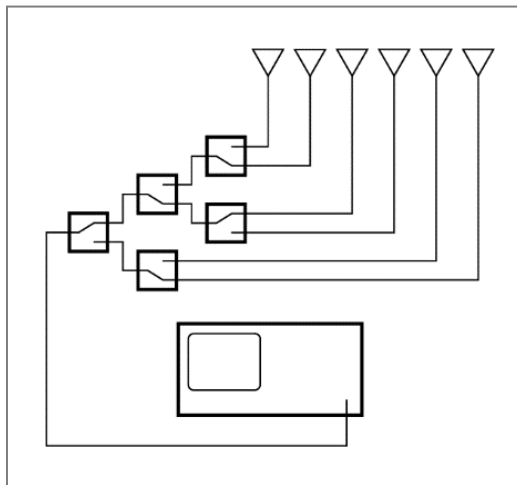
Figure 2. Tree matrix
