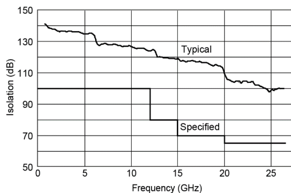
Figure 8. Isolation
