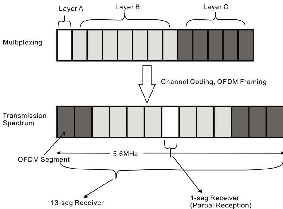
Figure 1. Hierarchical transmission and partial reception in ISDB-T
