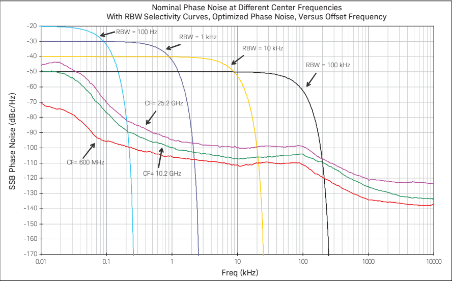
Figure 14. CXA-m (M9290A) nominal phase noise at different center frequencies
