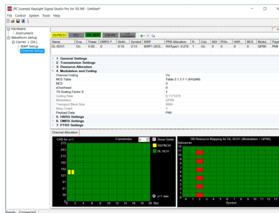
Figure 2: Signal Studio Pro 5G NR Channel Setup
