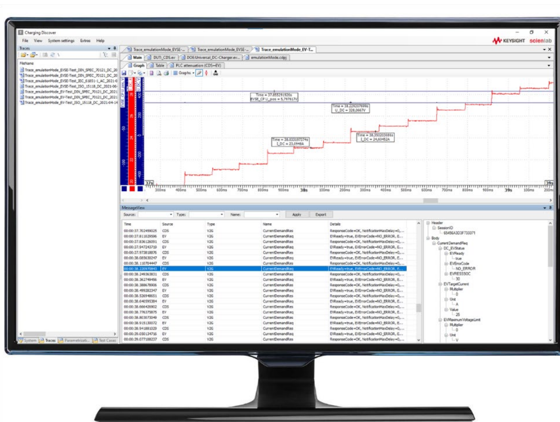
Figure 10. SL1300A Charging Discover Test Packages
