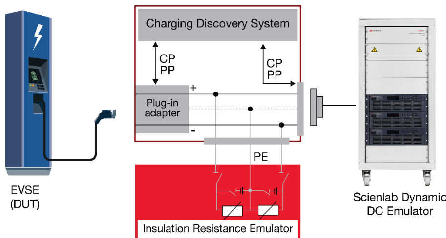
Figure 7. System topology including the SL1040A-IRE and SL1041B Scienlab Dynamic DC Emulator
