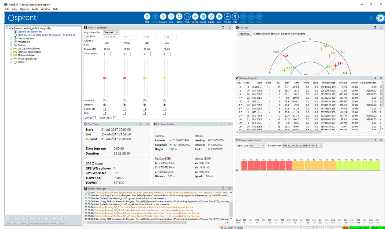
Figure 3. SimTEST main screen
