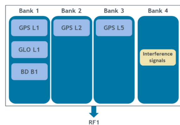
Figure 13. Triple-frequency, GNSS + interference 1RF system
