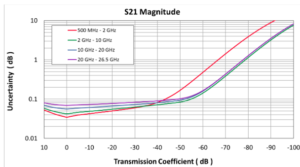
Transmission Uncertainty
