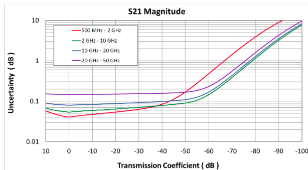
Transmission Uncertainty
