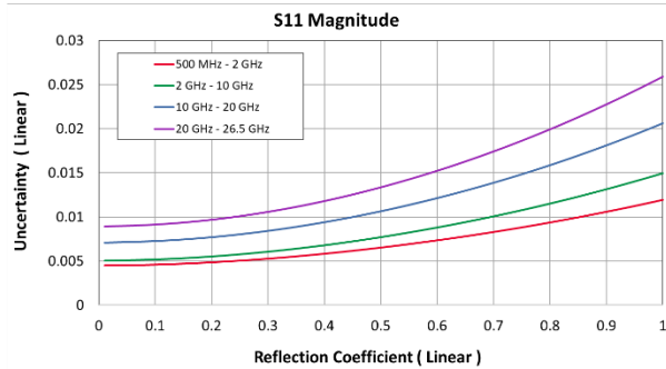
Reflection Uncertainty
