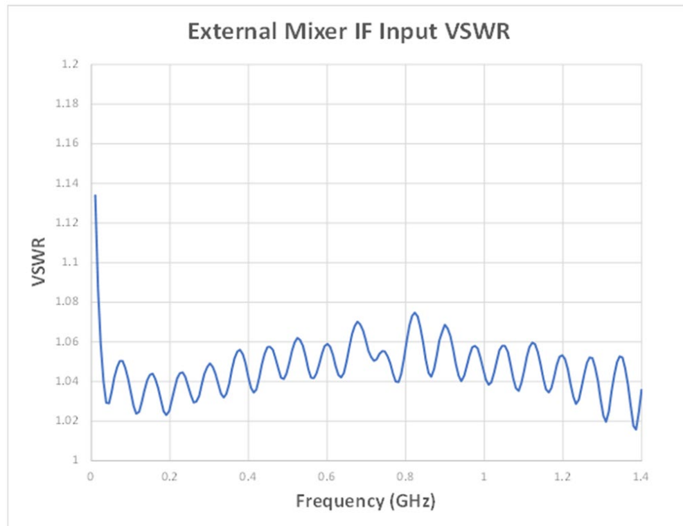
Figure 5. External mixer IF input VSWR
