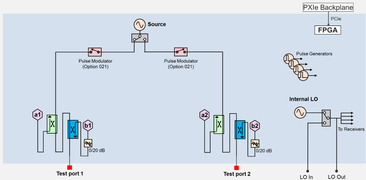
M981xA PXIe Receiver Module (Included in Option 491 or 691)
