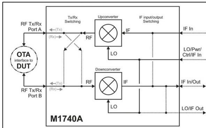
Figure 2. M1740A block diagram
