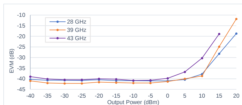
Figure 3. EVM vs. output power
