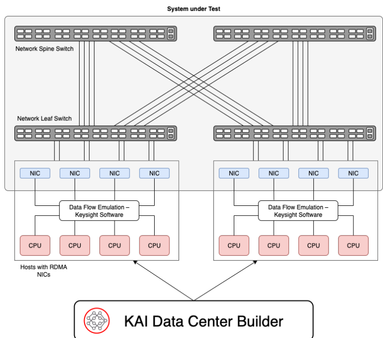
Figure 3. System Under Test Topology with Keysight software
