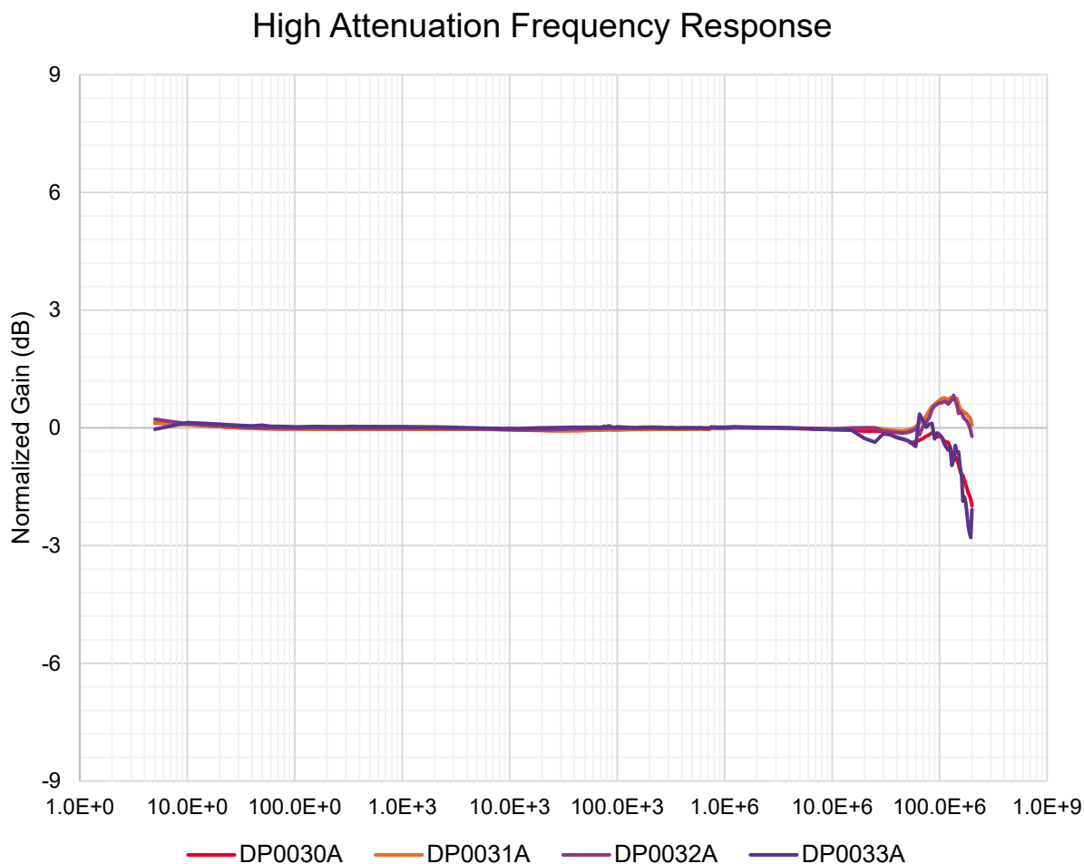
Figure 2. Vout/Vin frequency response of DP003xA probes on high attenuation settings.
