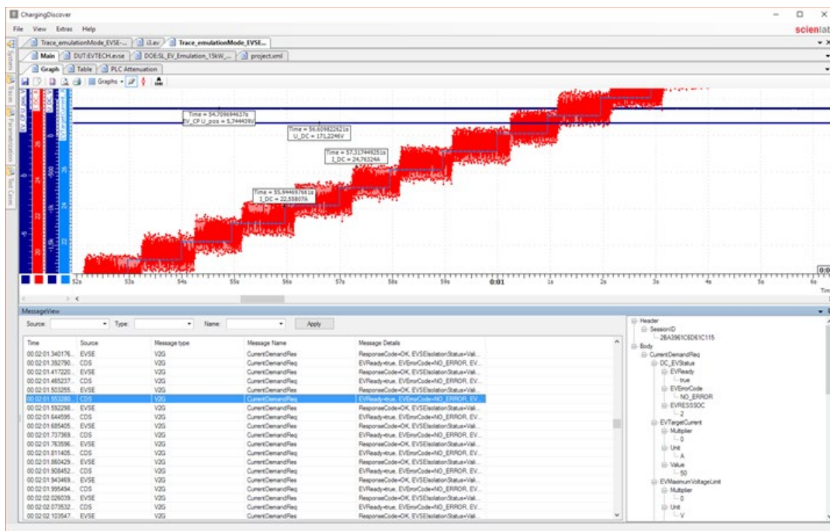
Figure 2. Traceability | Synchronous PWM, V2G and HV measurements, 1 ms resolution
