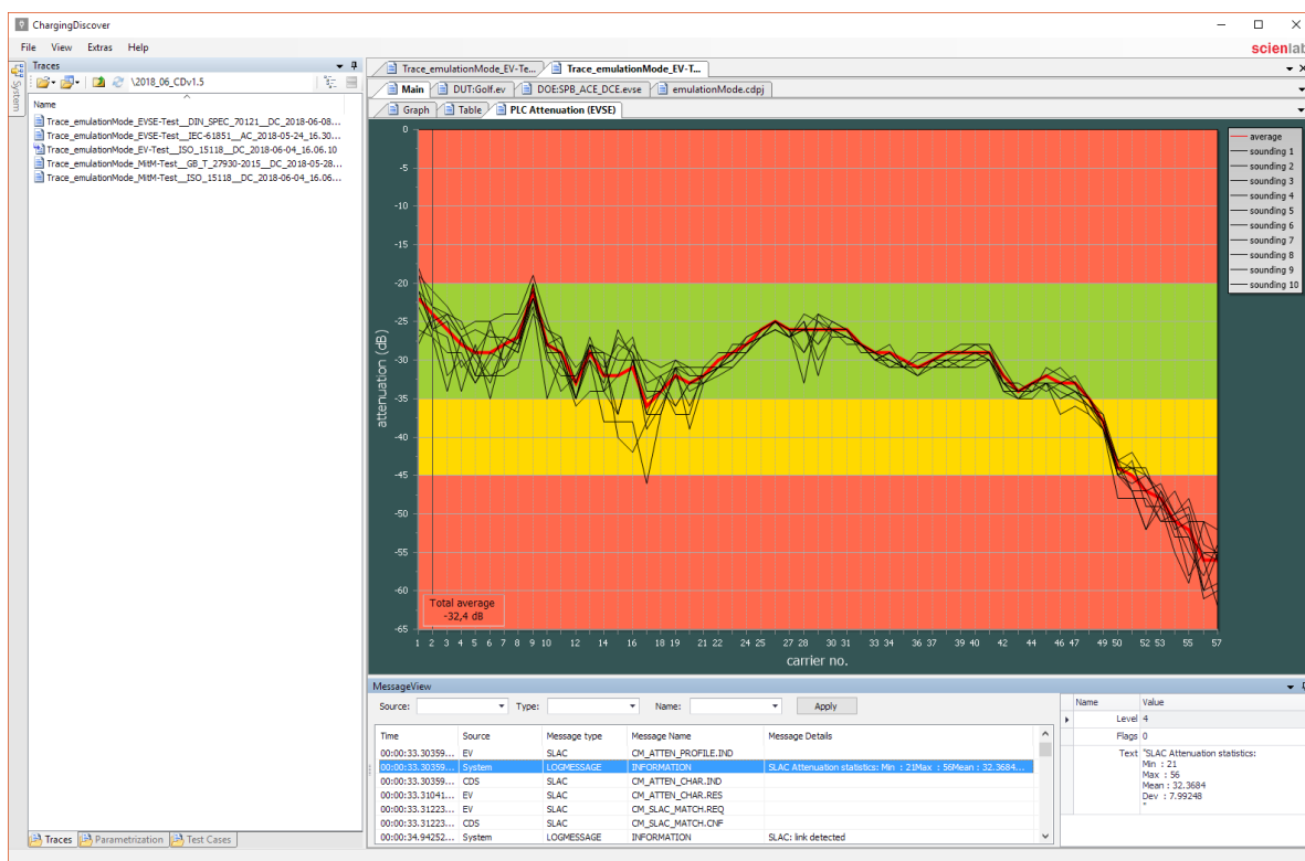
Figure 3. Traceability | Graphical SLAC attenuation
