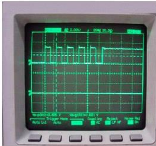
Figure 3. No cross-talk on adjacent channels.
