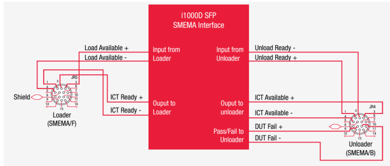
Figure 6. Medalist i1000D SFP inline SMEMA interface.
