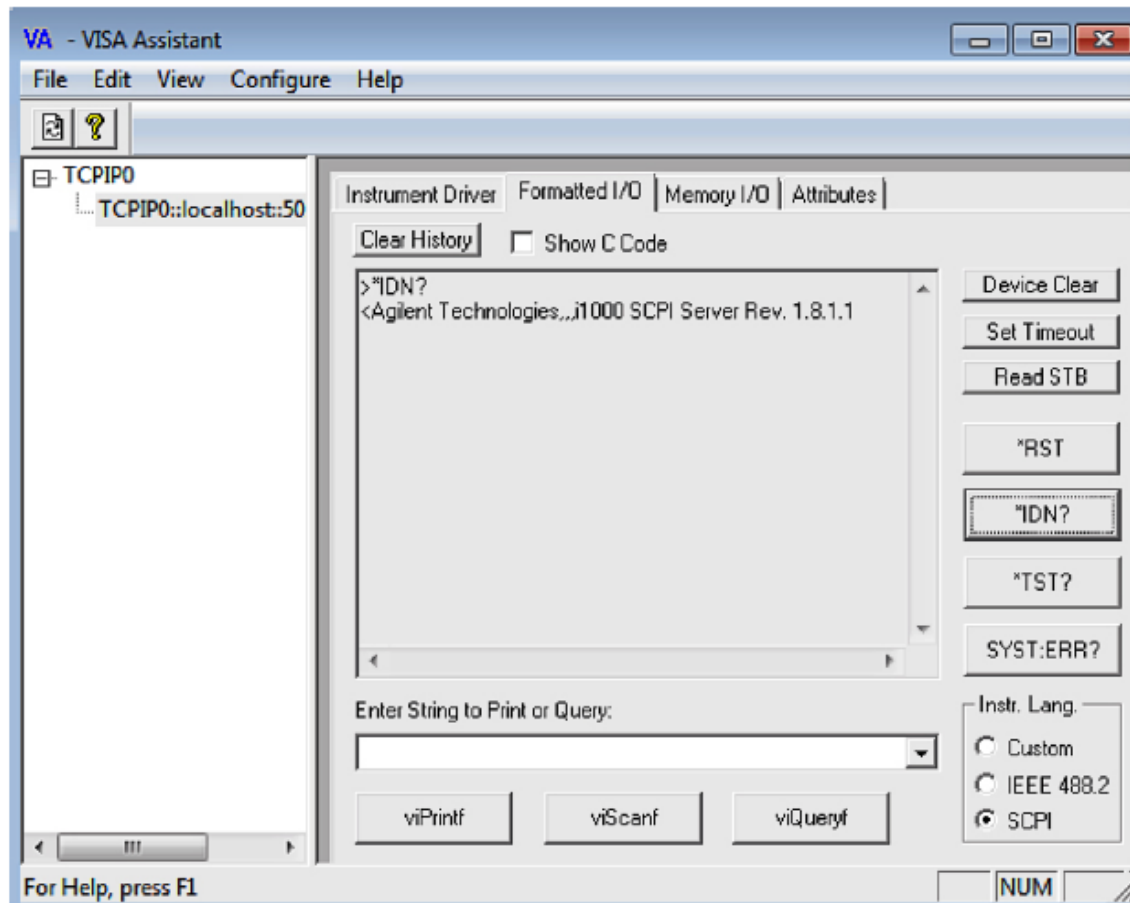
Figure 11. Running SCPI commands from VISA Assistant.
