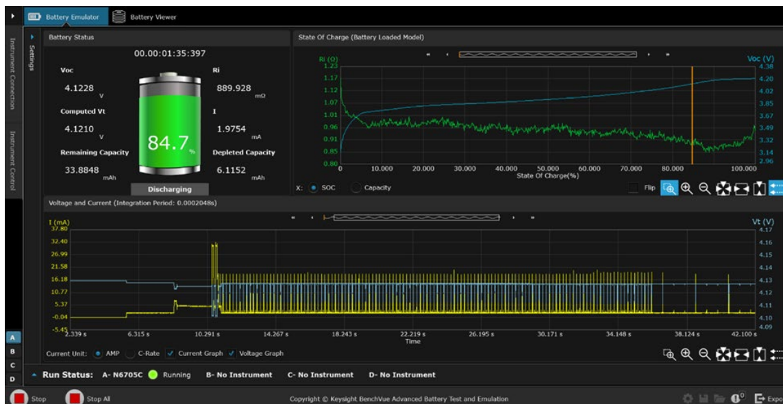
Figure 8. PW9253A connected to Keysight's advanced two-quadrant power supply
