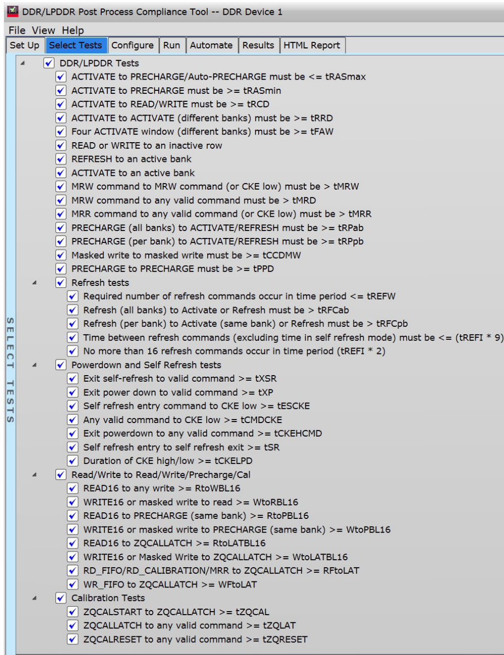
Figure 30. LPDDR4 post process compliance tests from B4661A Option -3FP/TP/NP.
