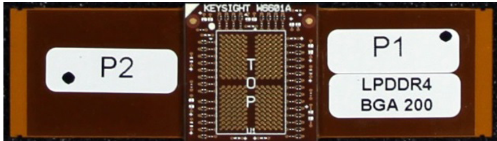
Figure 5. Top view of W6601A.
