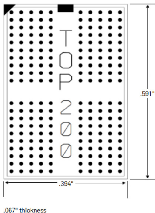
Figure 12. LPDDR4 200-ball riser. Dimensions in inches.
