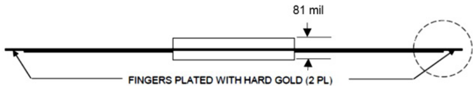
Figure 4b. W6601A side view.
