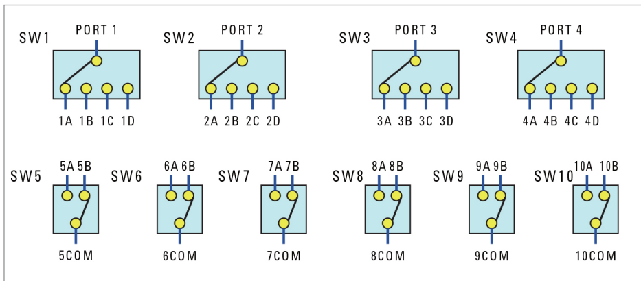
Figure 14. Switch configuration (E5092A-020)
