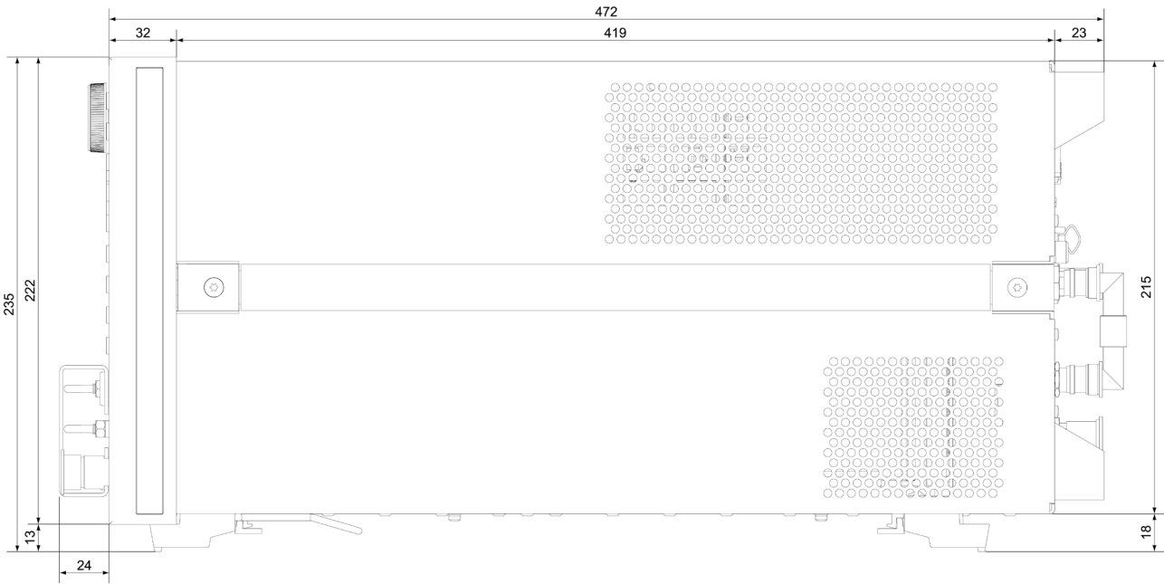
Dimensions (side view)
