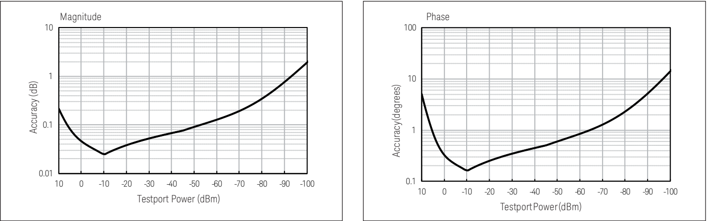
Figure 10. Dynamic Accuracy
