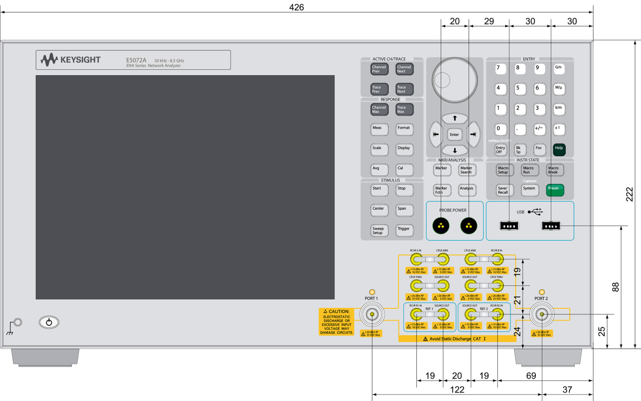
Dimensions (front view)
