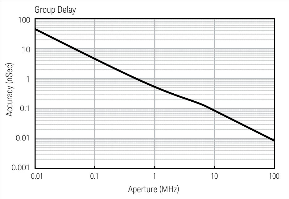
Figure 11. Group delay
