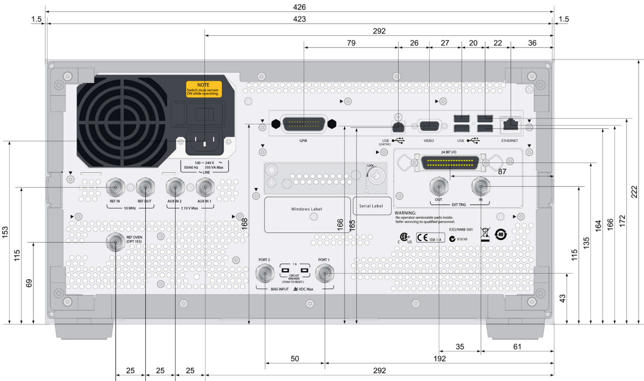
Dimensions (rear view)
