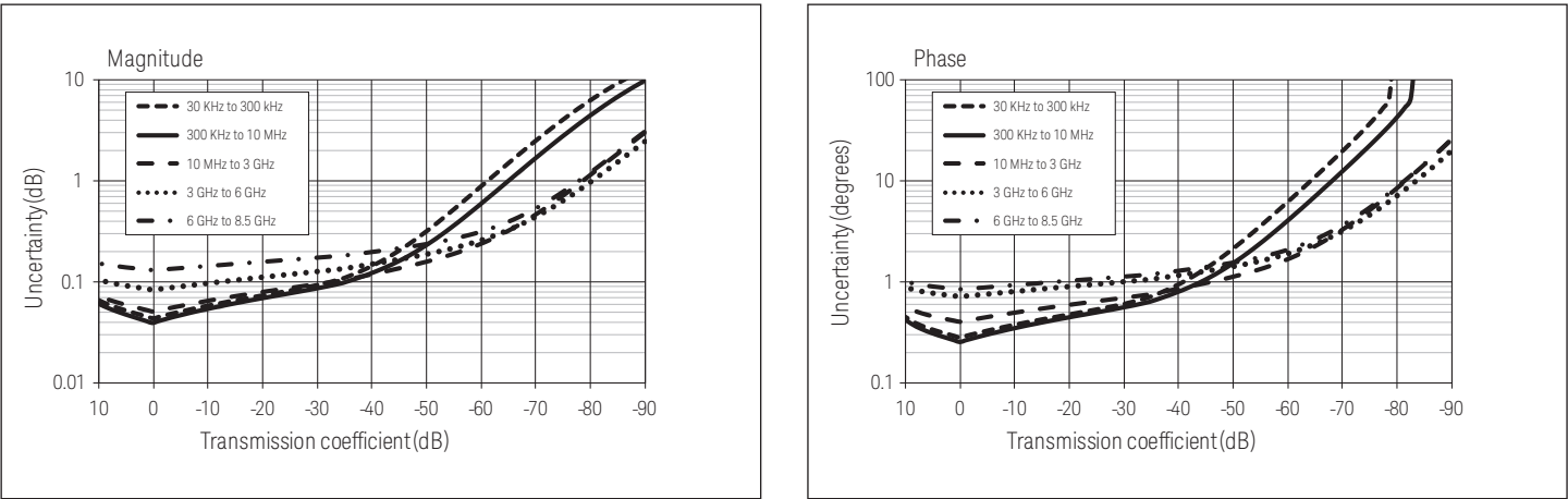
Figure 2. Transmission uncertainty (Specification)
