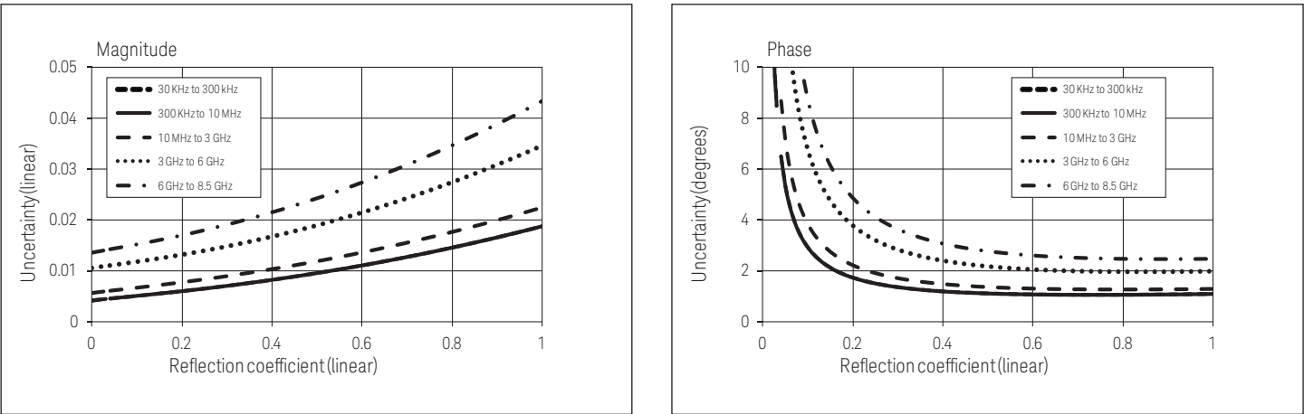
Figure 3. Reflection uncertainty (Specification)
