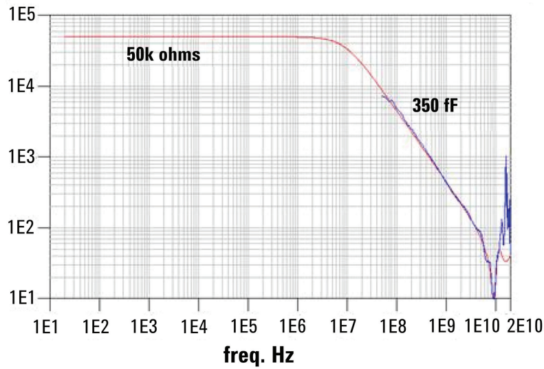
Figure 3 Differential Input Impedance plot, input C = \sim 0.72 pF
