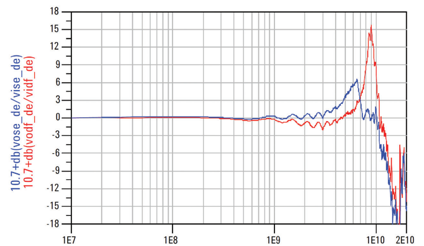
Figure 2 Frequency response of the N2887A, red = Single-ended, blue = Differential
