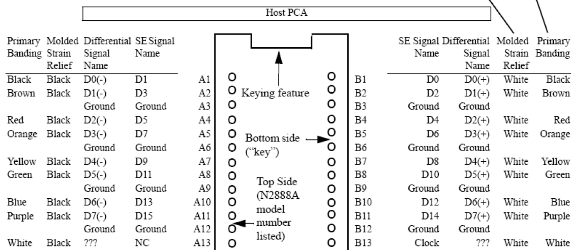
Figure 7 Pin assignment map of the N2888A InfiniiMax Soft touch half-channel adapter
