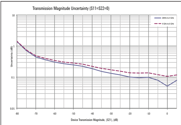
Figure 6: Transmission uncertainty
