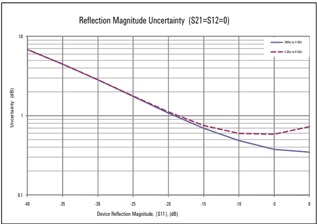
Figure 7: Reflection uncertainty
