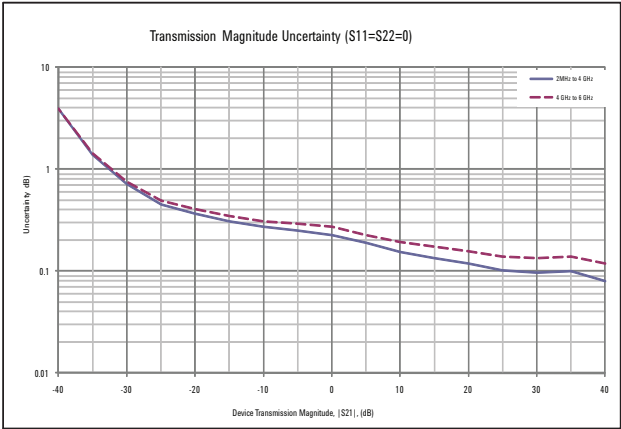
Figure 8: Transmission uncertainty
