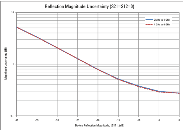
Figure 3: Reflection uncertainty (specification)
