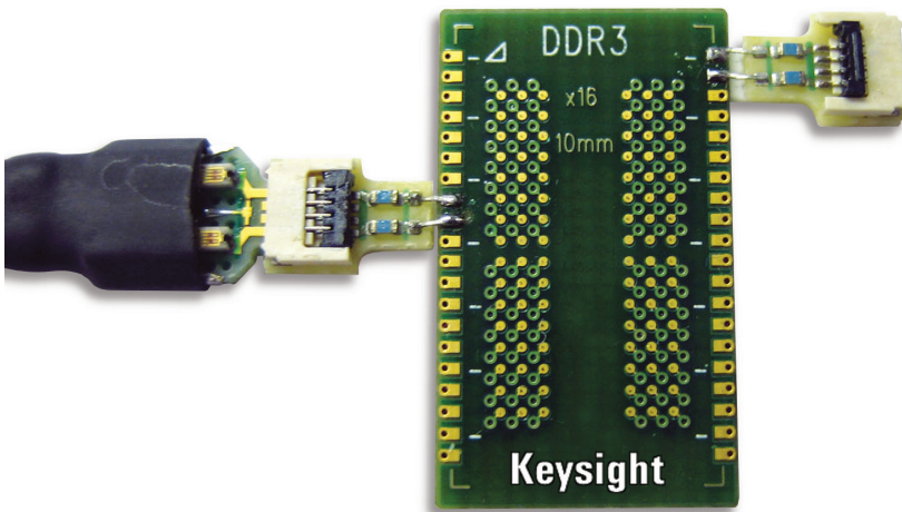
Figure 2. The picture above shows the InfiniiMax N5425A and N5426A ZIF probe head connected to the W2636A DDR3 BGA probe adapter.
