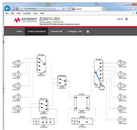
Figure 25. Interactive RF schematic using Z2091C Smart Switch
