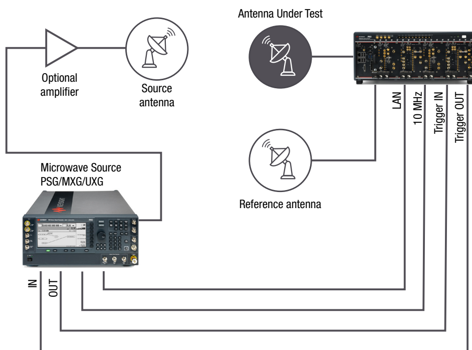
Figure 14. Multiport phased array antenna test setup
