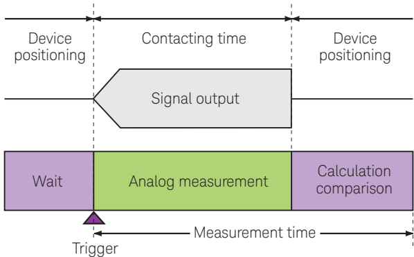
Figure 5. Synchronous source
