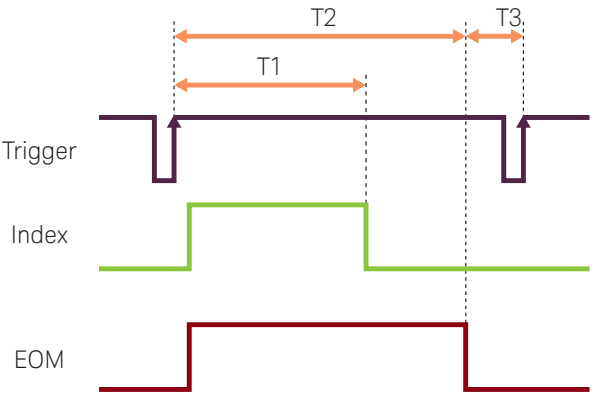
Figure 1. Measurement speed
