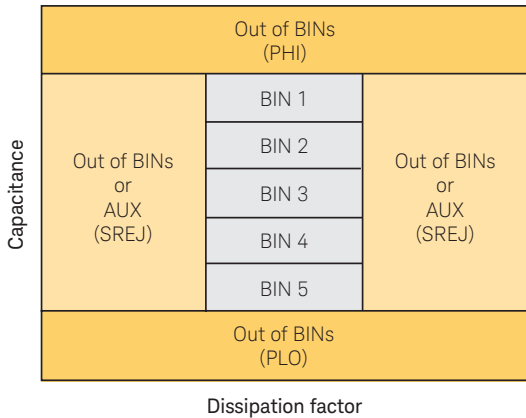
Figure 3. Bin sorting
