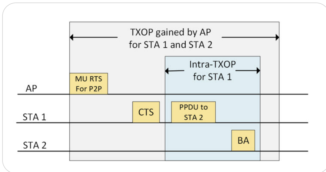
Figure 13. Triggered P2P operation
