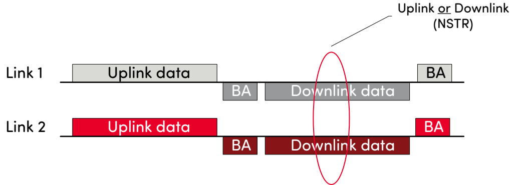
Figure 19. Non-simultaneous synchronous operation NSTR
