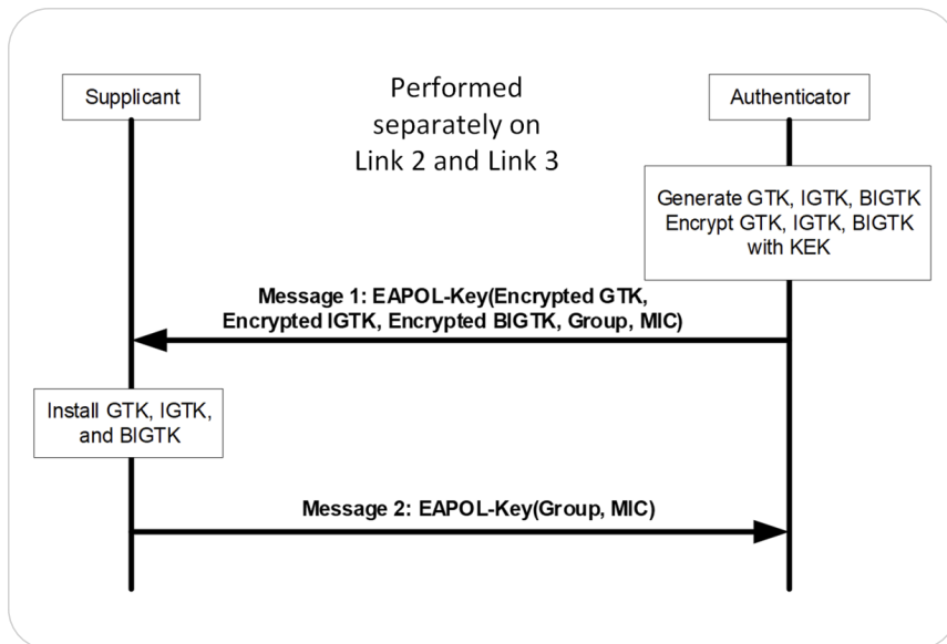
Figure 24. Group key handshake
