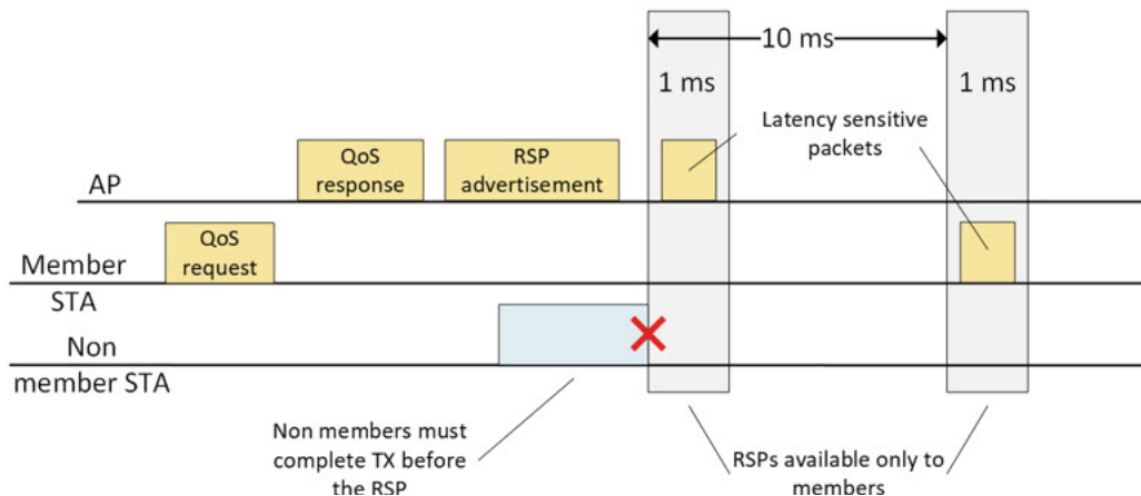
Figure 10. Enhanced QoS using restricted service periods
