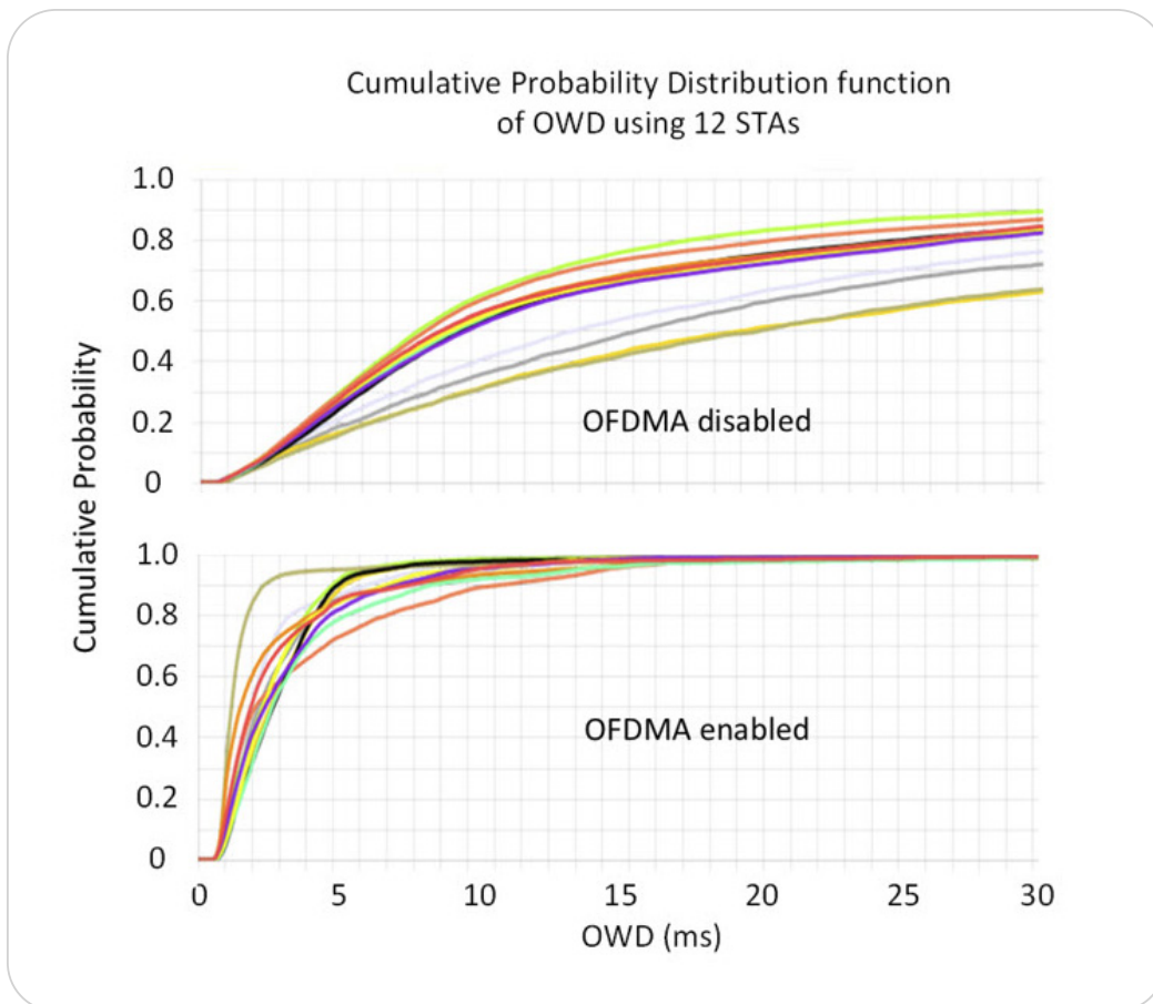
Figure 9. Wi-Fi 6 latency improvement compared to legacy
