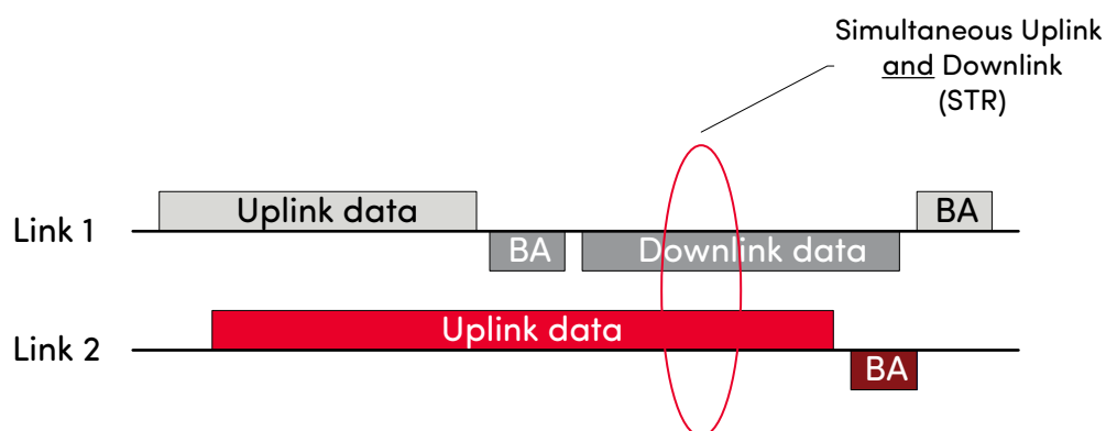
Figure 18. Simultaneous asynchronous operation STR
