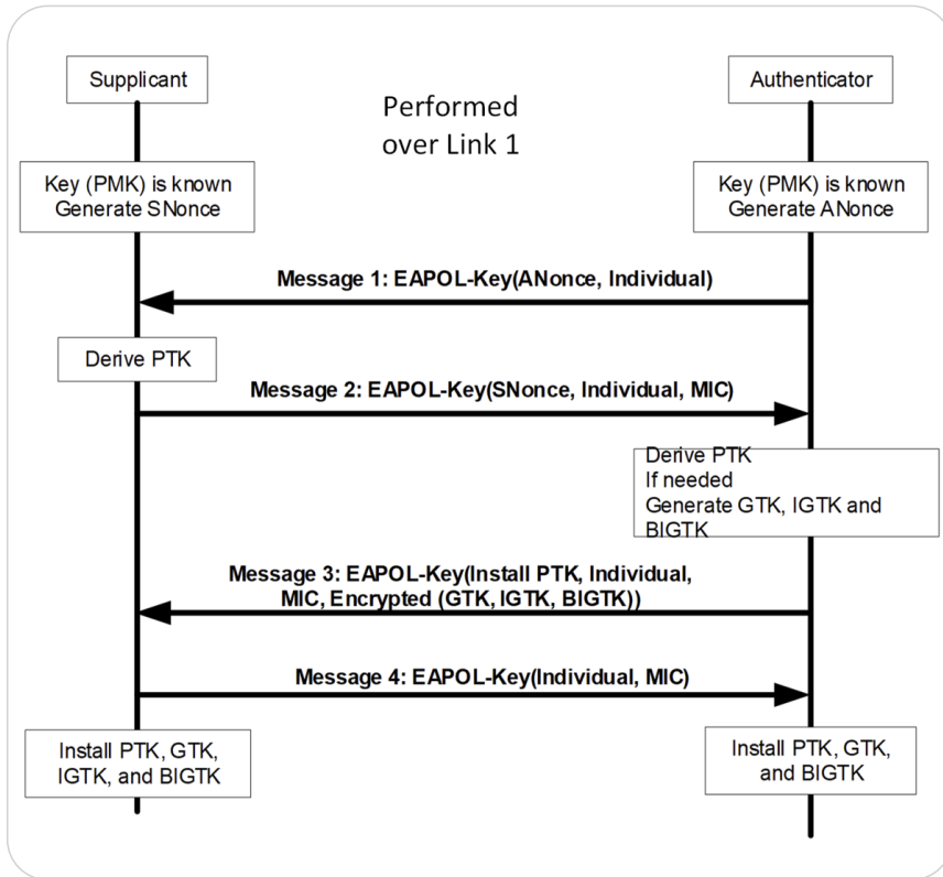
Figure 23. Four-way handshake for security setup
