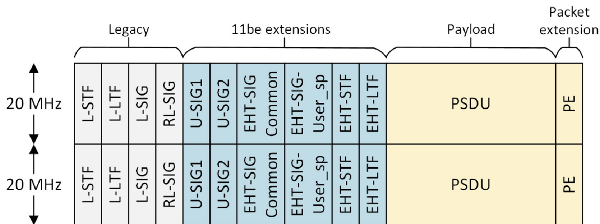
Figure 4. EHT preamble
