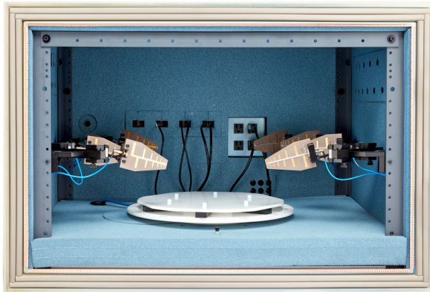
Figure 26. Octobox small anechoic chamber with turntable
