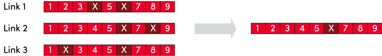
Figure 16. MLO for increased reliability
