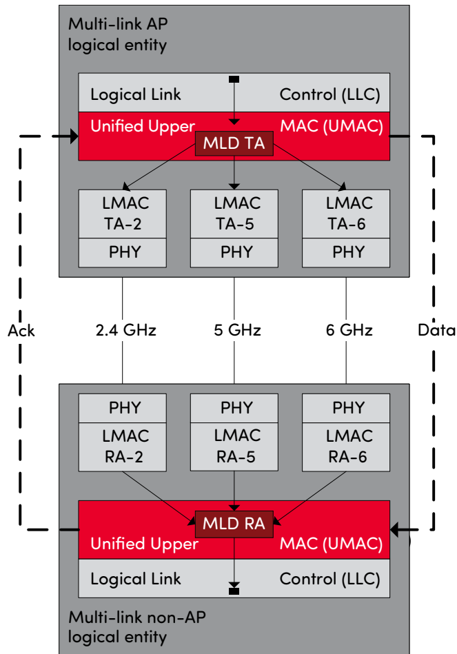
Figure 14. MLD architecture
