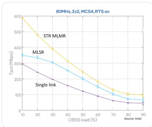
Figure 20. Performance comparison of different MLDs
