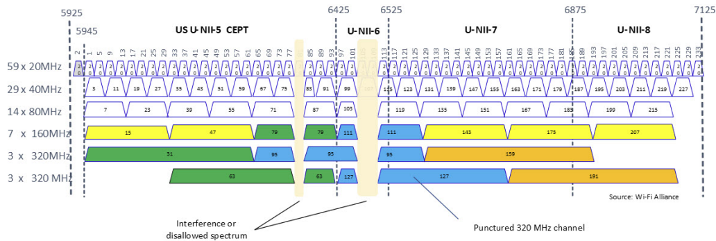
Figure 6. Illustration of puncturing
