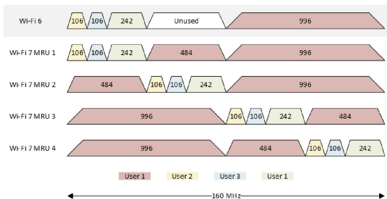
Figure 7. Examples of Multi RU operation
