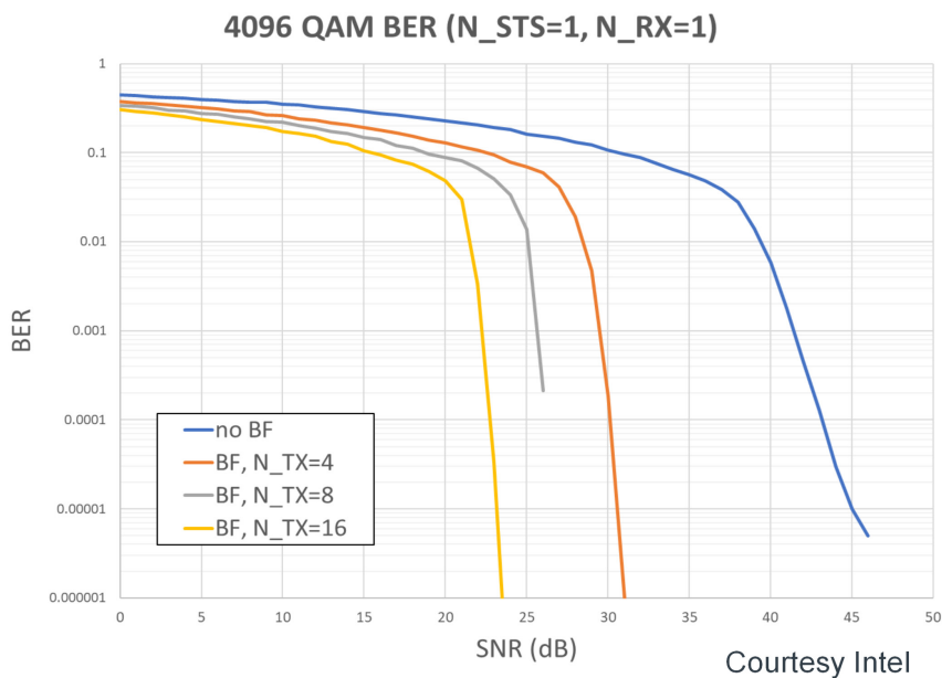
Figure 3. Diversity gains using multiple antennas
