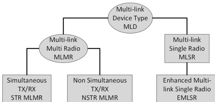
Figure 17. Multi-link device hierarchy
