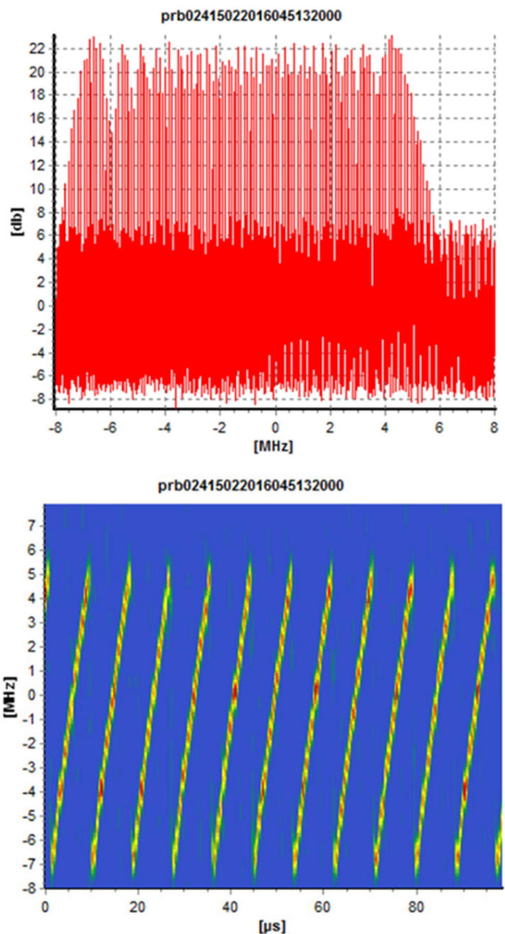
Figure 3. Sawtooth jamming waveform detected by Keysight near an airport in Germany
