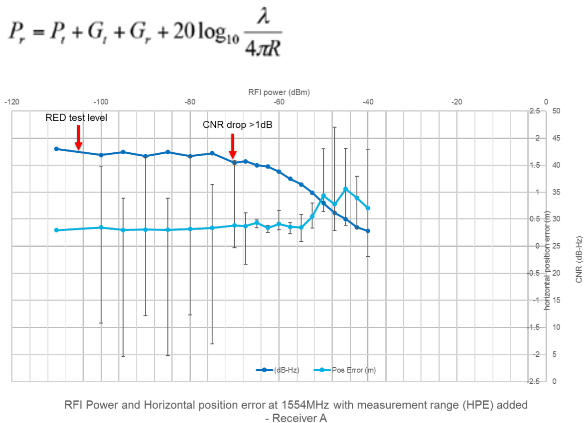
Figure 4. Observed effects of adjacent-band interference on HPE in a GPS L1 receiver
