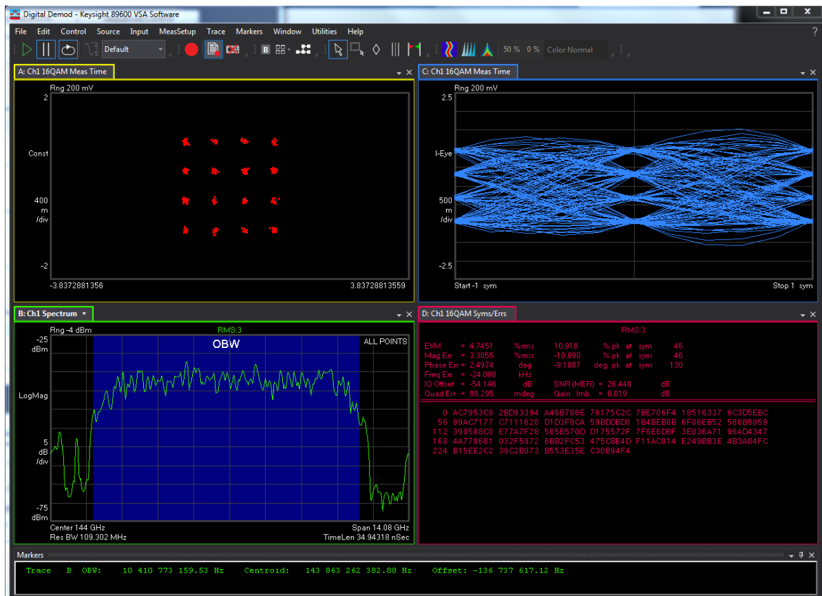
Figure 12. 16 QAM OTA measurements performed at 144 GHz with G-band VDI converters, 10 GHz occupied bandwidth
