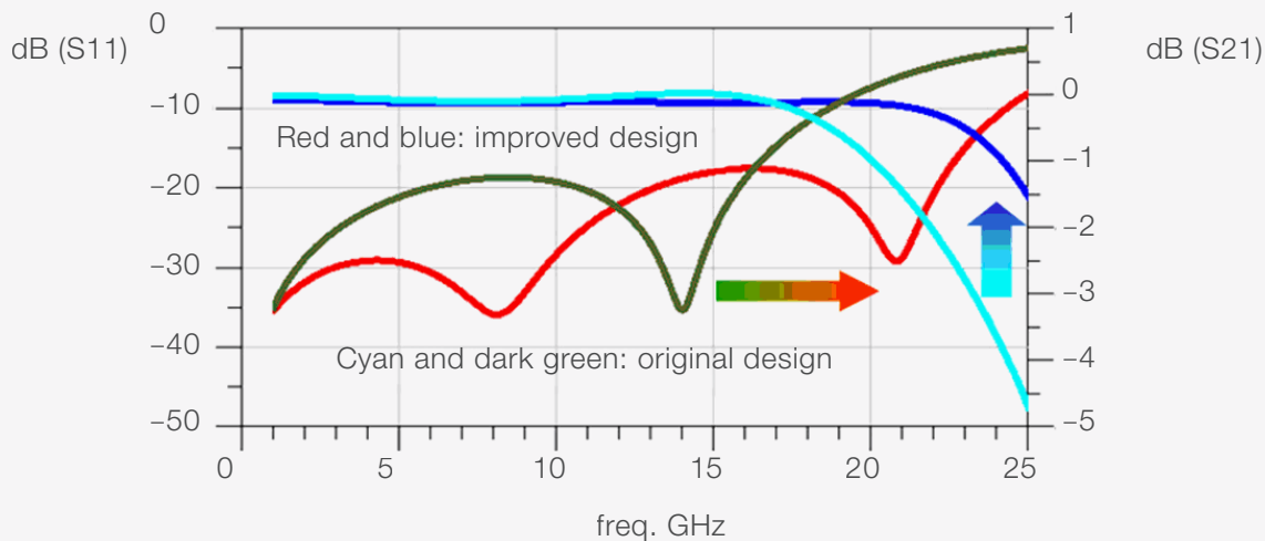
Figure 7. Improved QFN package performance
