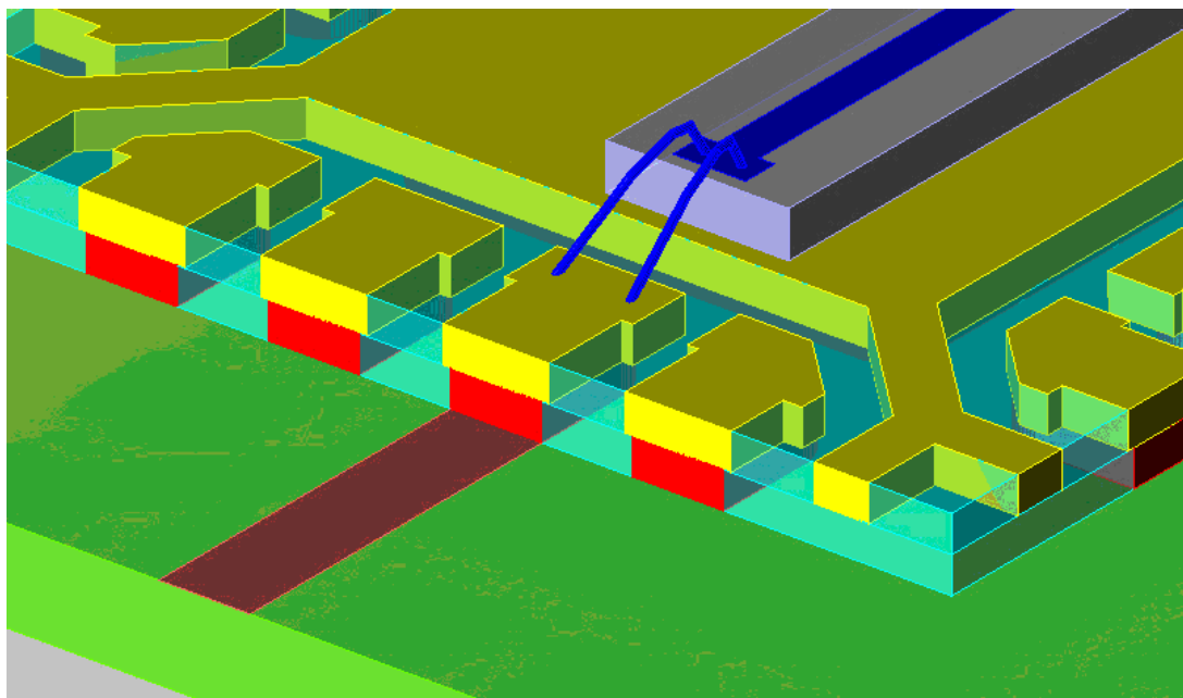
Figure 6a. Original design
