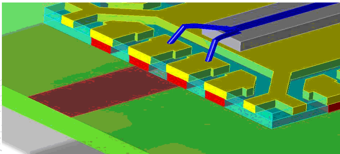
Figure 6b. Improved transition design
