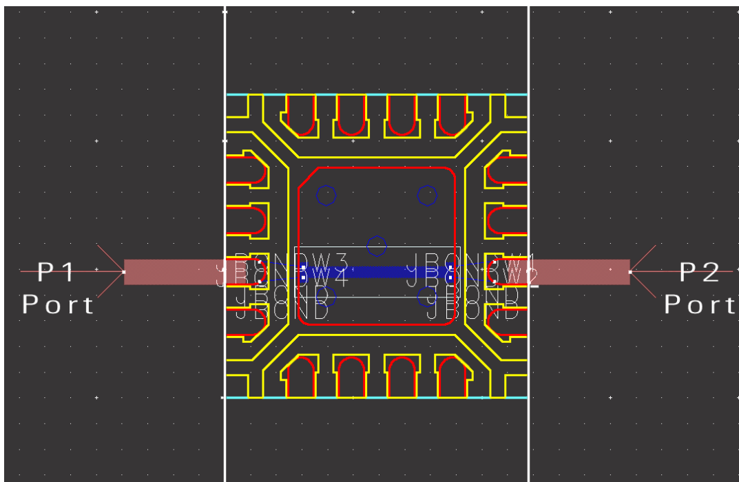
Figure 5. ADS layout of QFN package on PCB
