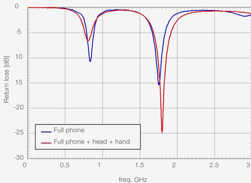
Figure 8. Distortion of the mobile-phone's return loss in the proximity of a head and hand
