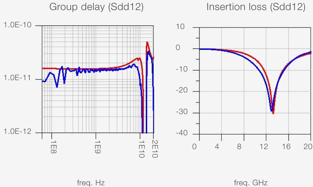
Figure 3. Simulated (red) and measured (blue) group delay and insertion loss
