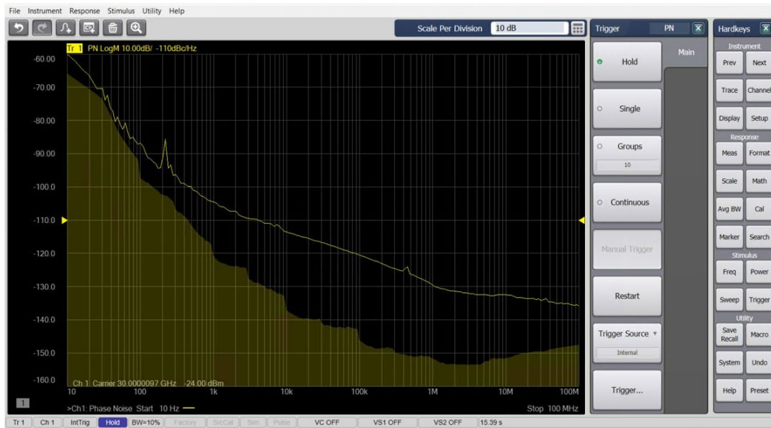
Figure 12. Phase noise measurement with SSA-X
