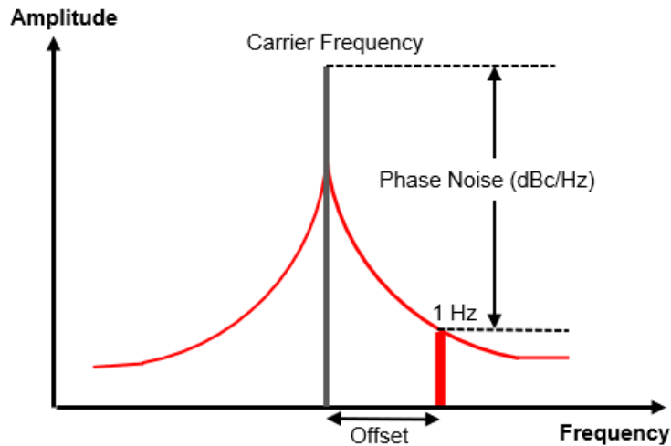
Figure 3. Single-sideband phase noise
