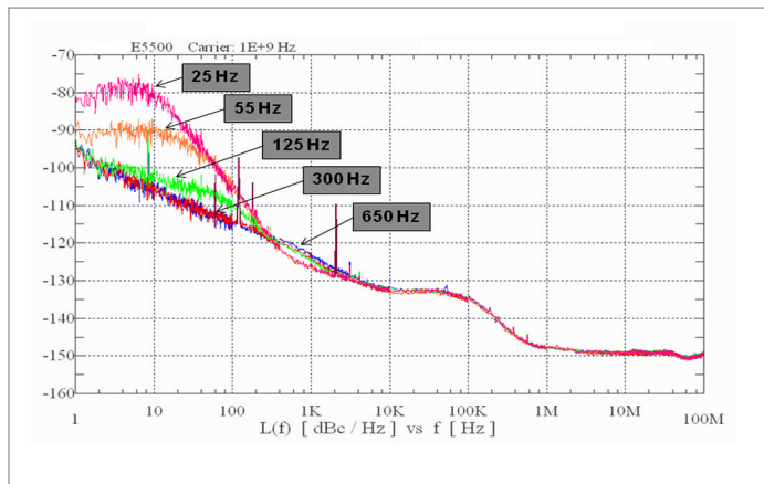
Figure 7. Each bandwidth setting provides visible changes in PSG phase noise
