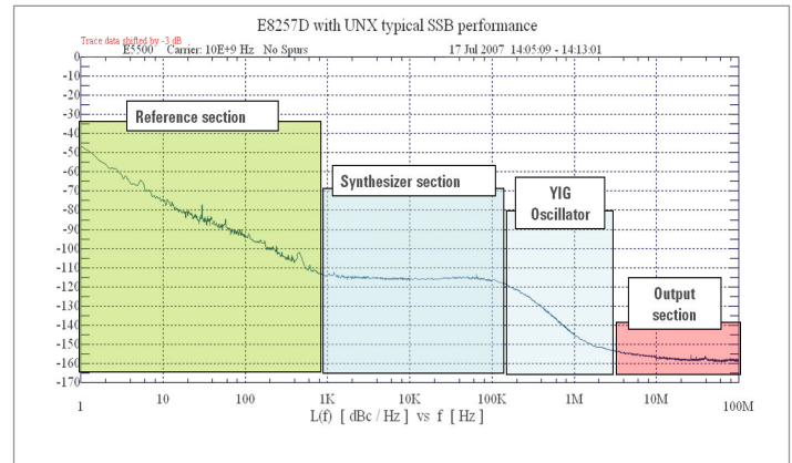
Figure 2. Each section of the instrument block diagram is the dominant contributor to an identifiable portion of phase noise performance
