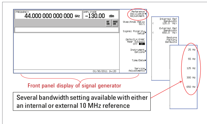
Figure 6. Bandwidth adjustments are accessed through front-panel soft menus in the PSG
