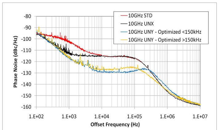
Figure 9. Modes 1 and 2 provide improved phase noise performance in the pedestal region (1 kHz to 100 kHz)
