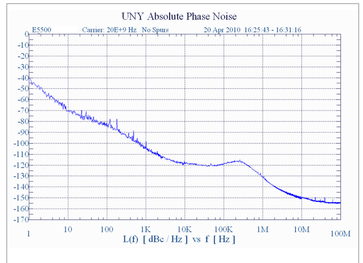
Figure 1. An example of a log-log plot that shows phase noise at a carrier frequency of 20 GHz
