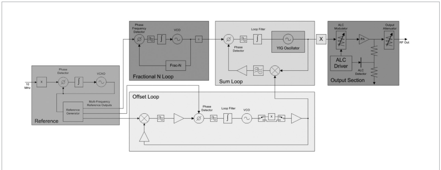
Figure 3. Keysight's triple-loop architecture enables tremendous improvements in phase noise performance
