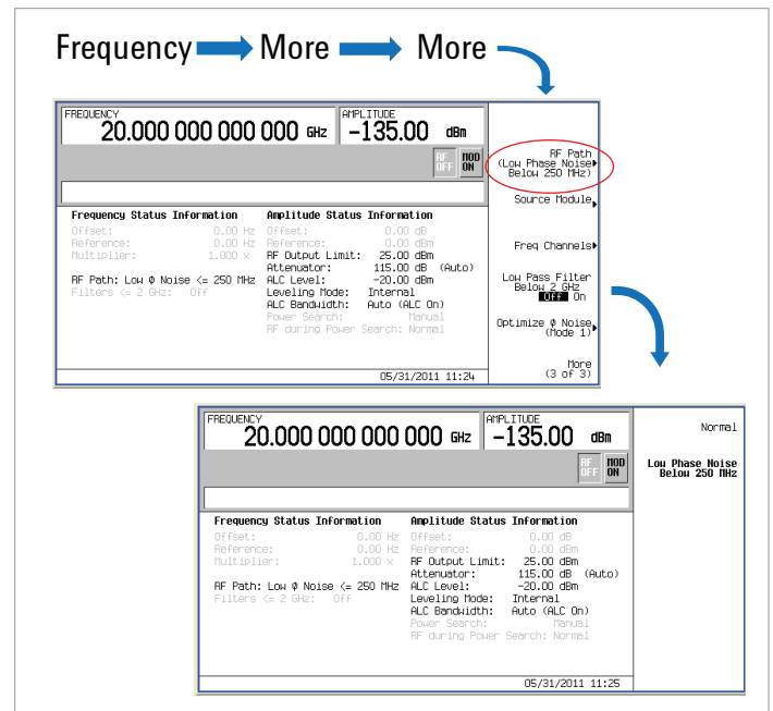
Figure 10. The "RF Path (Low Phase Noise Below 250 MHz)" function activates the divider mode
