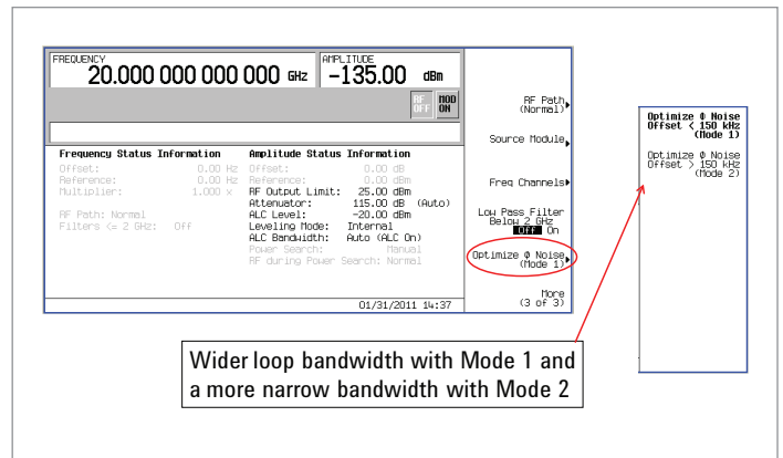
Figure 8. The "Optimize Noise" function provides two modes that affect YIG oscillator loop bandwidth
