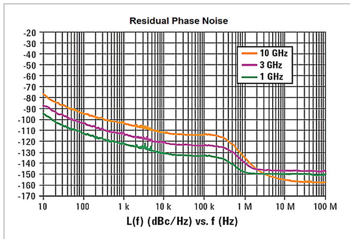
Figure 4. Residual phase noise represents the phase noise of the signal generator, excluding the reference section. This is in contrast to absolute phase noise, which represents the generator's total phase noise.
