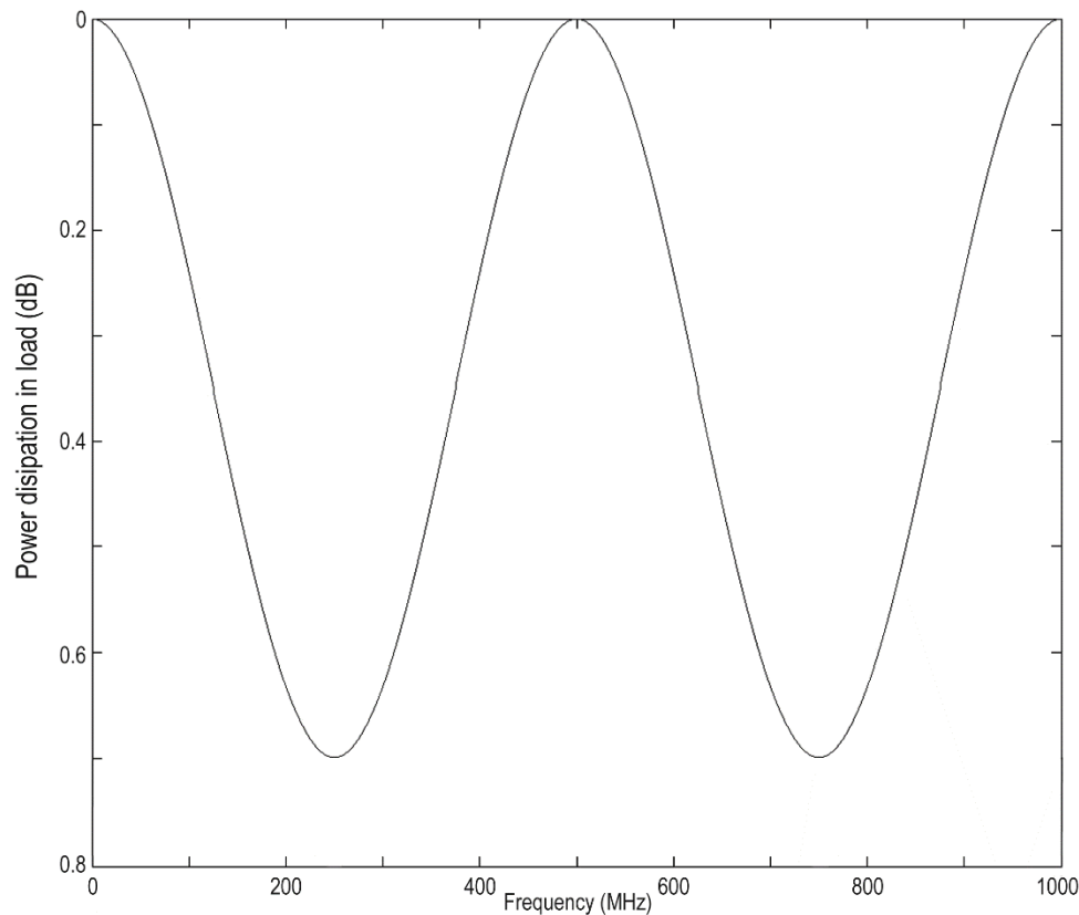
Figure 3-4. Even a short (8-in) length of 75- \Omega transmission line connecting two 50- \Omega systems causes regular variations of power with frequency, with a peak excursion of 0.7 dB. All this is below 1000 MHz.
