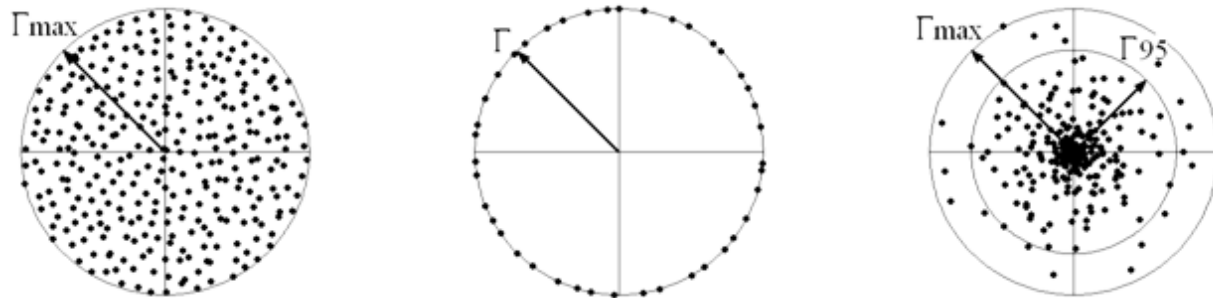
Figure 4-3. When the reflection coefficients of the generator and load are not known, the user may estimate probabilities of the mismatch uncertainty according to these cases:
