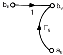
Figure 2-3. Signal flowgraph of a microwave generator
