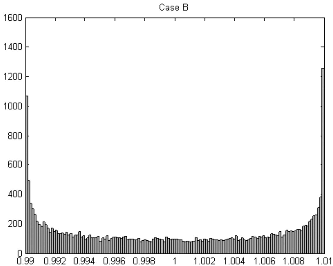
Figure 4-5. Histogram of M_u for case B, two rings distribution, showing the U-shaped distribution.
