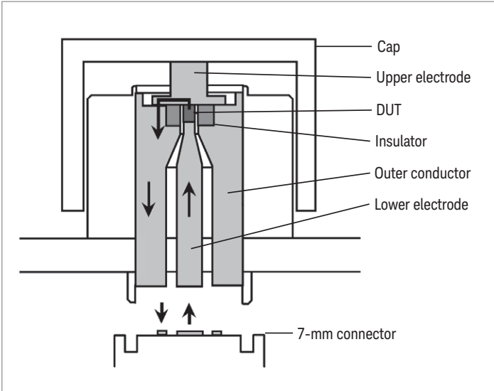
Figure 8. Cross-sectional drawing of the test fixture structure
