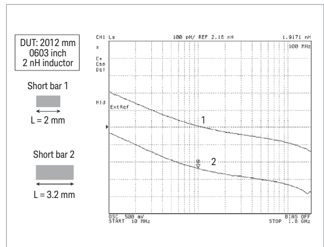
Figure 3. Necessity of using the same sized short bar
