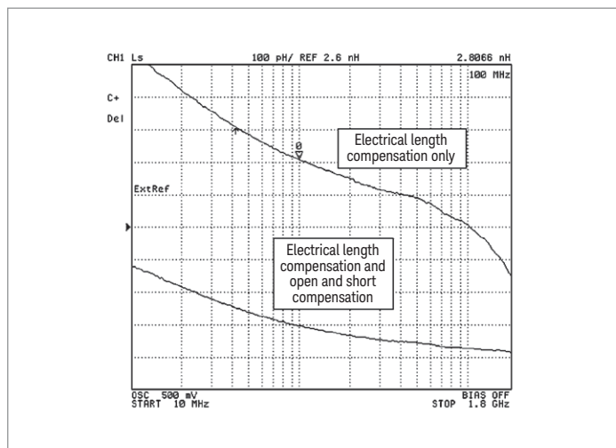
Figure 2. Difference in measurement results caused by a difference in compensation method. xture
