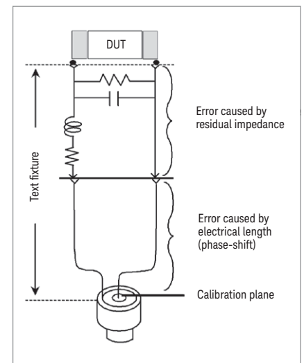
Figure 1. Residual error model of test fixture
