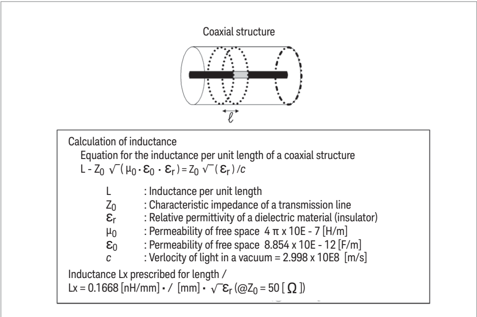
Figure 9. Theoretical derivation of the short plate’s residual inductance
