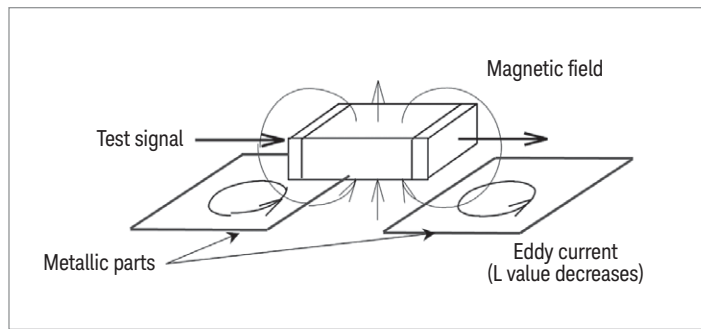
Figure 7. Influences from the surrounding structure of the DUT
