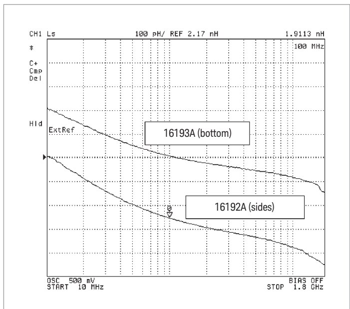
Figure 6. Difference in contacting from the sides and from the bottom
