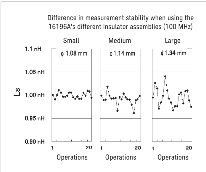
Figure 12. Measurement stability improvement when using appropriate insulator assembly
