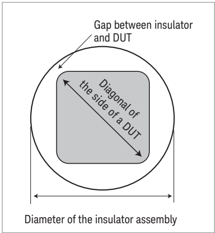
Figure 11. Gap between insulator and DUT
