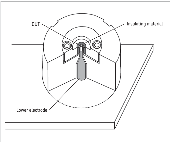
Figure 13. Cross-sectional drawing of 16196A/B/C/D
