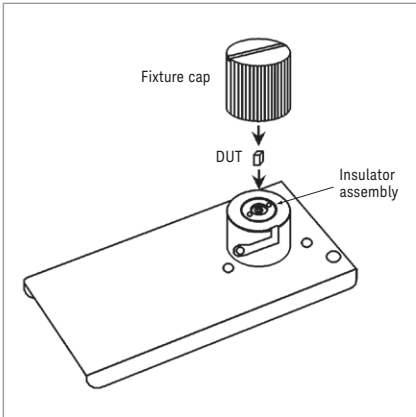
Figure 10. Positioning of the DUT
