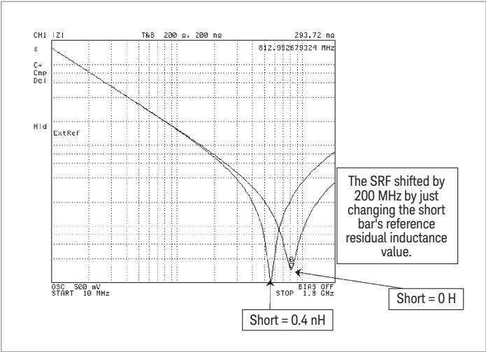
Figure 4. Capacitor ‘s SRF shifted due to the short bar’s residual inductance value
