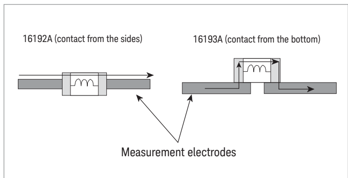
Figure 5. Changes in the test current's path due to the position of measurement electrodes
