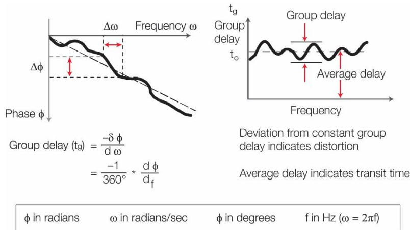
Figure 14. What is group delay?
