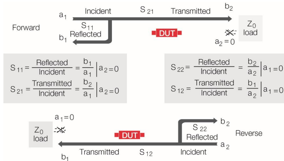
Figure 17. Measuring S-parameters
