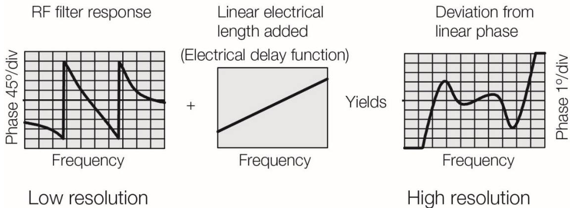
Figure 13. Deviation from linear phase
