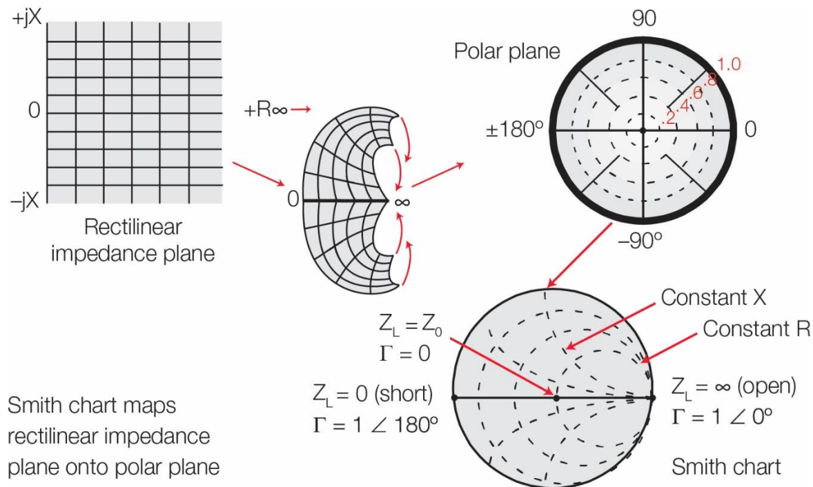
Figure 6. Smith chart review
