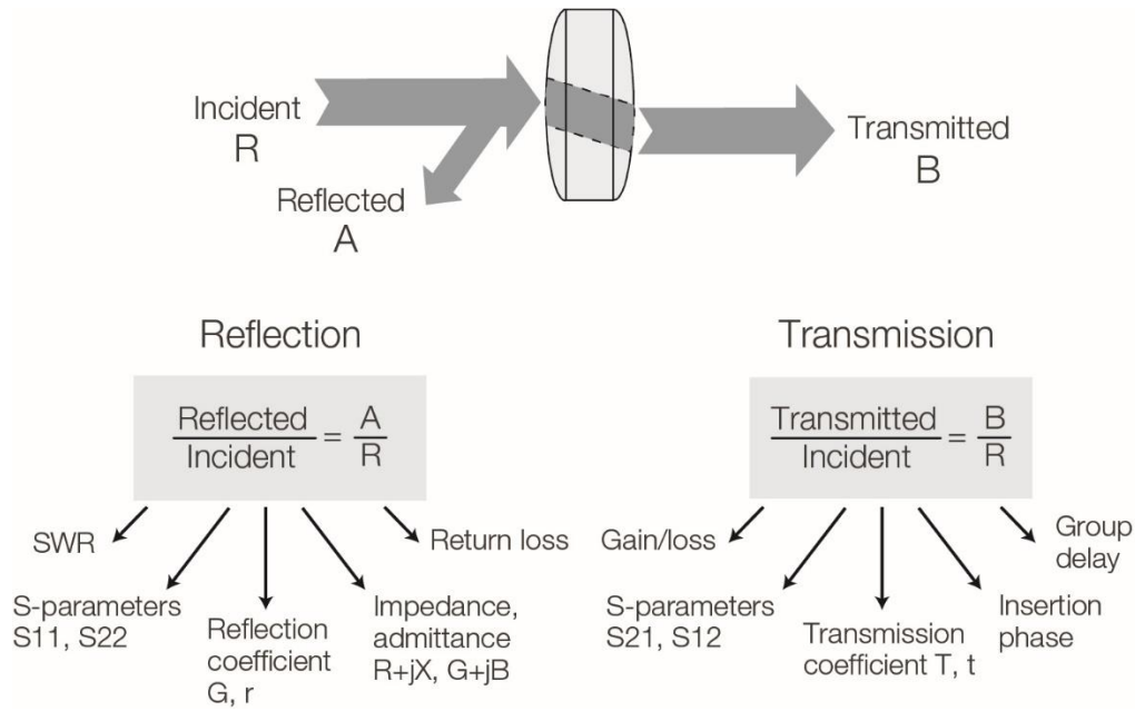
Figure 10. Common terms for high-frequency device characterization
