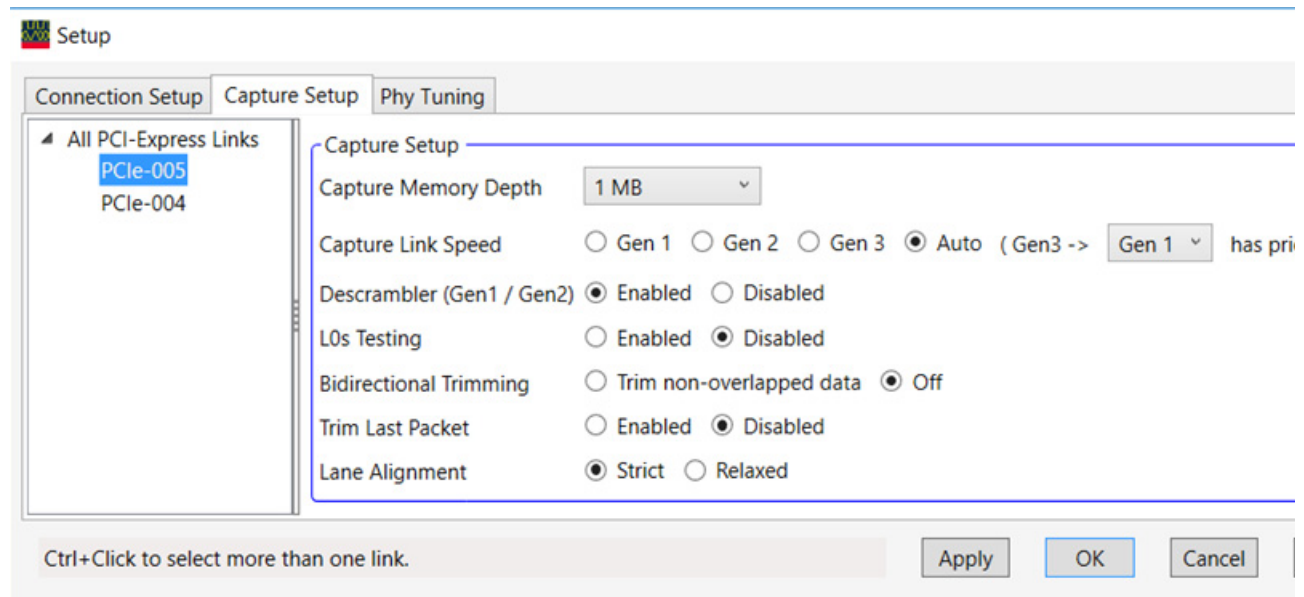
Figure 2 Capture Setup
