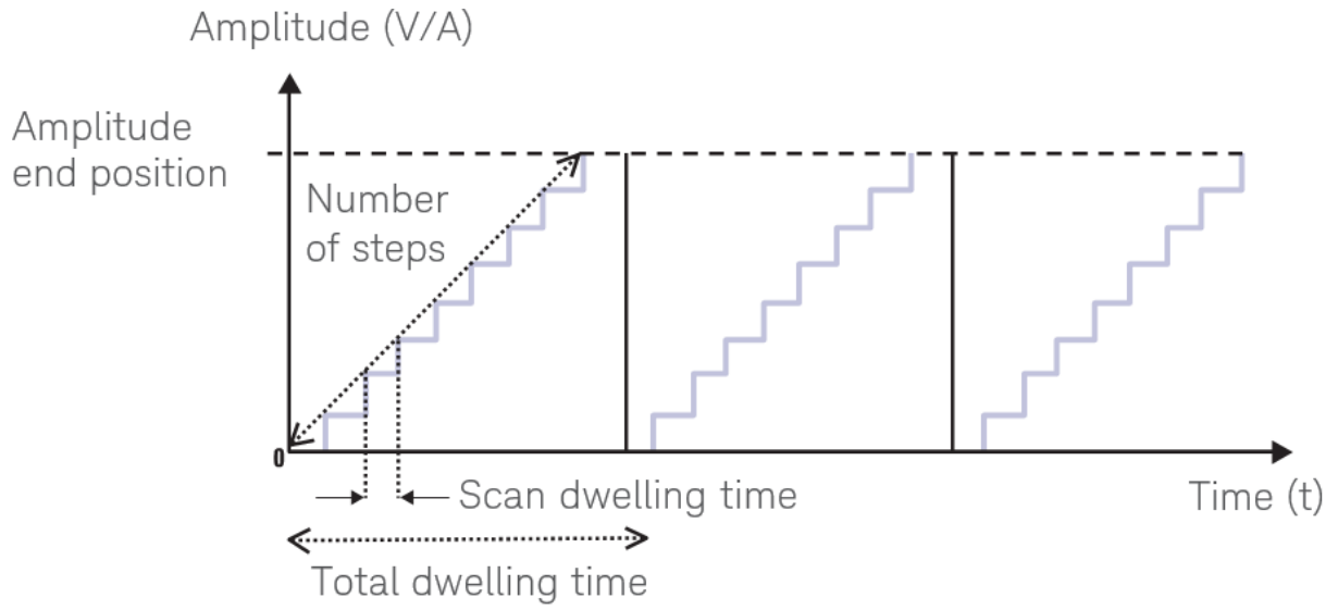
Figure 1. Scan Signal
