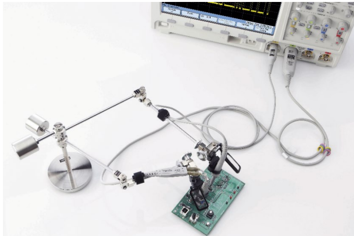
Figure 2. N2785A two-arm probe positioner
