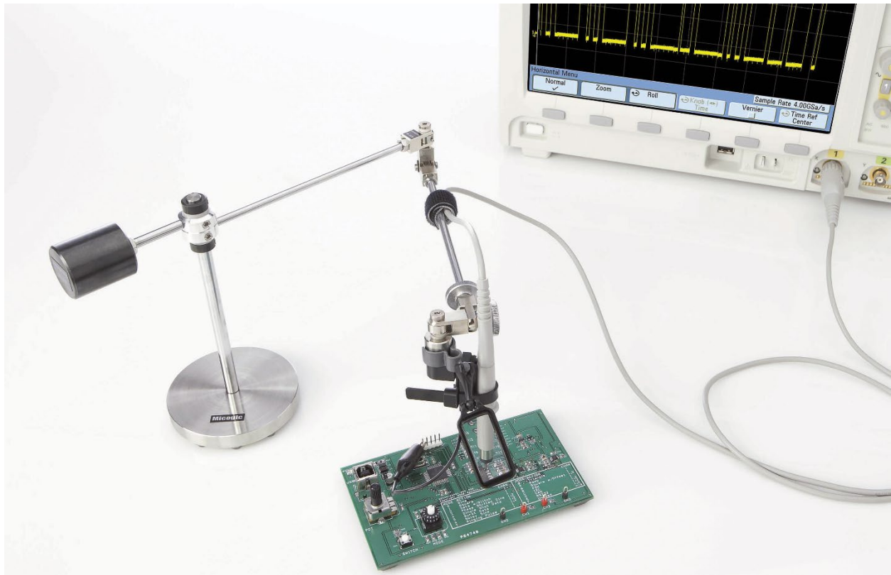
Figure 1. N2784A one-arm probe positioner
