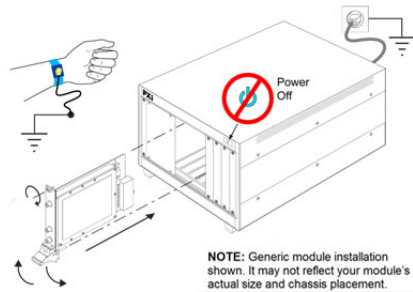
Figure 8 Depiction of installing a PXIe embedded controller
