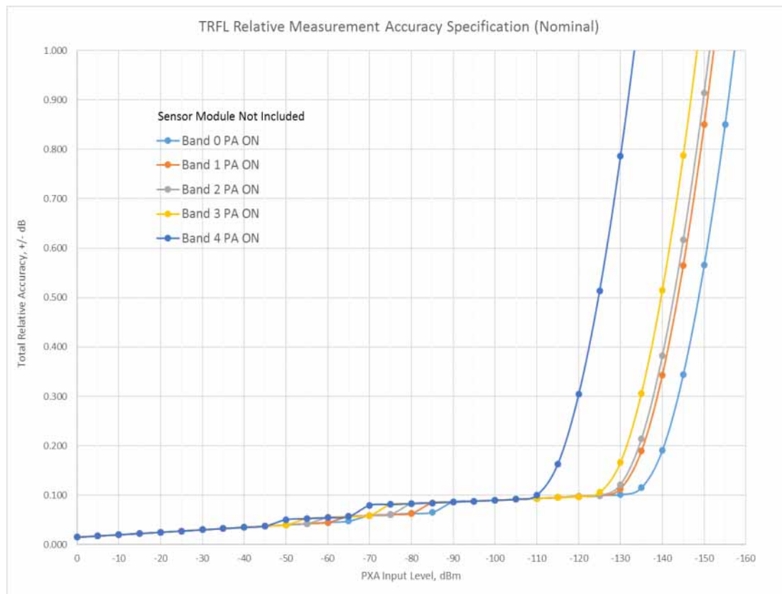
N9030B, Option 503/508/513/526, IF BW 10 Hz – Preamp On: Option P03/P08/P13/P26 [Plot]
