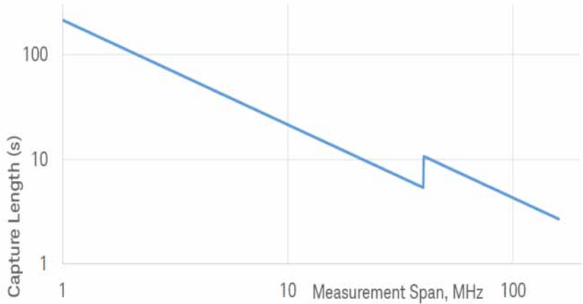
Capture Length versus Span, with Auto Bit Packing
