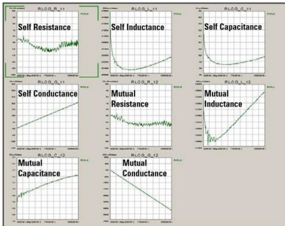
Figure 23. RLCG model extraction (W-Element shown).
