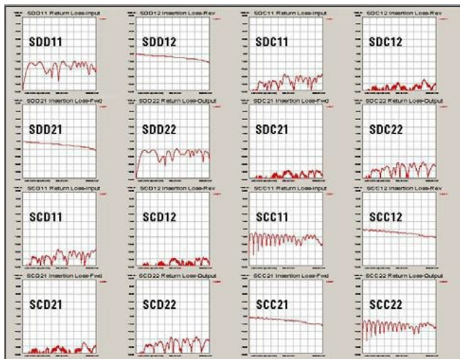
Figure 14. The mixed-mode frequency-domain matrix.
