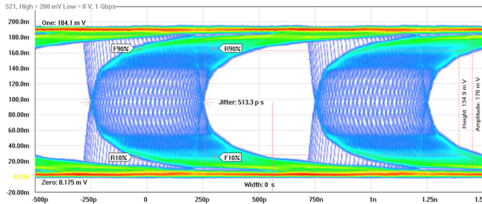
Figure 17. Choose StatEye virtual PRBS pattern for faster eye diagram generation of long patterns
