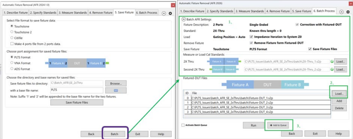
Figure 26. Batch AFR automation simplifies the repetitive AFR setup process on by de-embed multiple channels with one fixture model.
