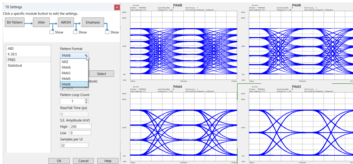
Figure 25. Pulse amplitude modulation, PAM-N eye formats for high data rates signal analysis.
