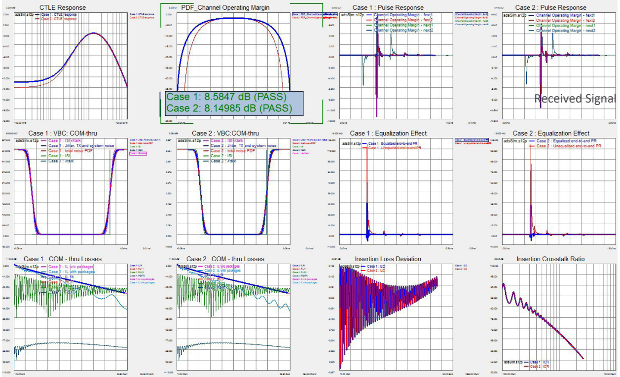
Figure 24. Channel Operating Margin (COM) testing inside PLTS platform enables design engineer to make interoperability trade-off studies to maximize performance/cost ratio in high-speed digital channels.
