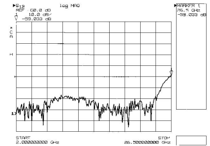
Figure 4. Reverse isolation measurement
