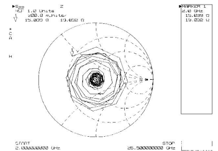
Figure 8. Complex output impedance measurement
