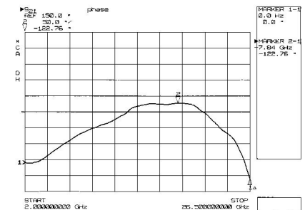
Figure 5. Deviation from linear phase measurement
