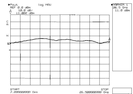
Figure 11. Absolute output power measurement
