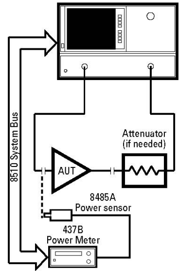
Figure 9. Power flatness correction setup
