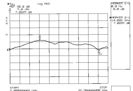
Figure 3. Small signal gain measurement
