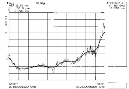
Figure 6. Group delay measurement with minimum and increased aperture
