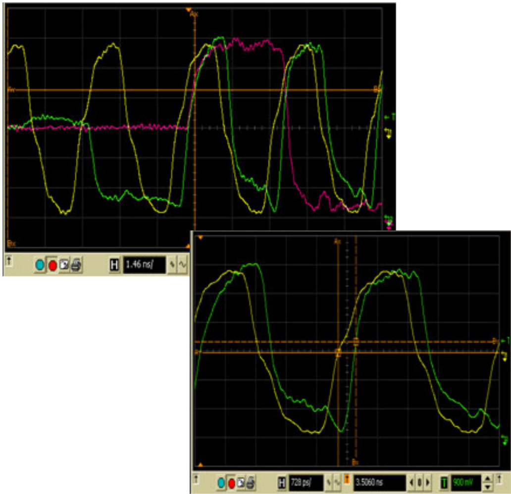
Figure 40 tDQSCK in Infiniium oscilloscope
