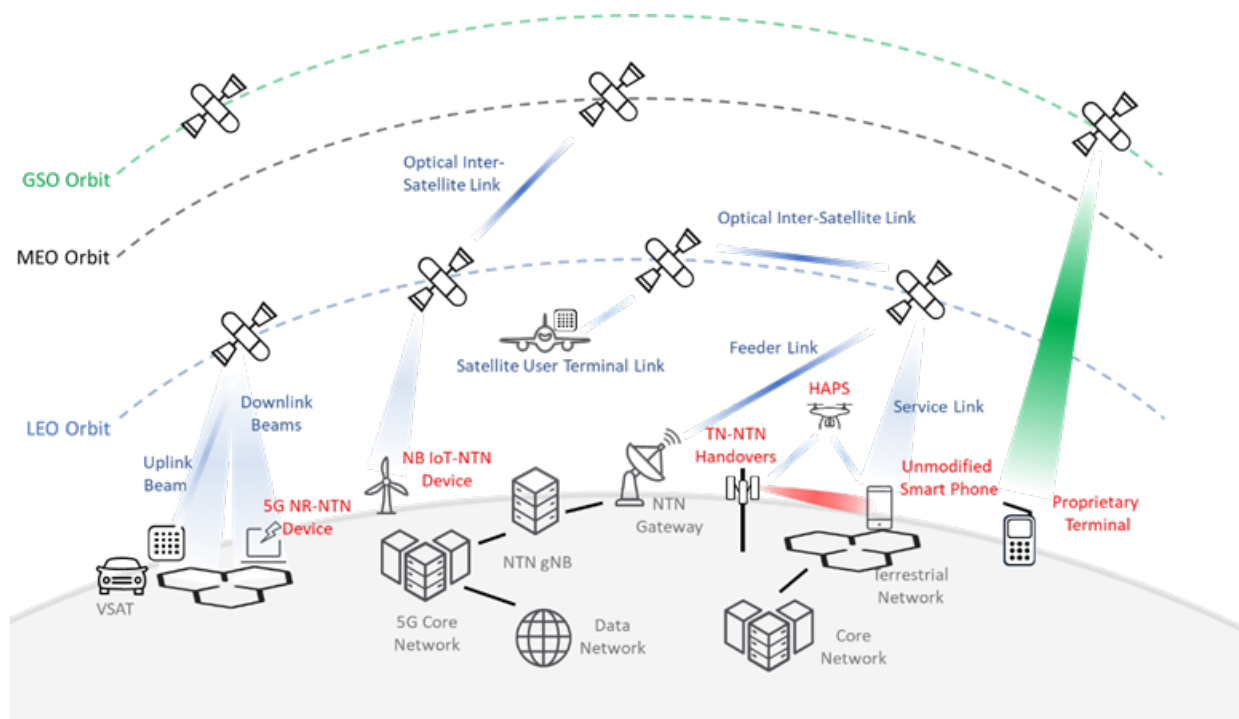
Figure 4. Integration of terrestrial and non-terrestrial networks
