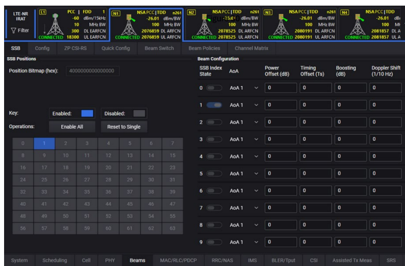
Figure 30. Flexible beam management configuration
