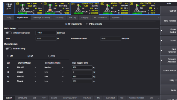
Figure 12. Baseband fading channel model configuration
