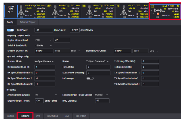
Figure 24. PC5 Sidelink
