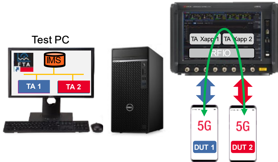
Figure 22. Two UEs connected end-to-end with one UXM 5G
